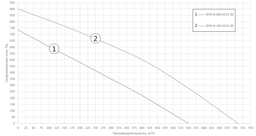
ZPVR-N HE EC NC
