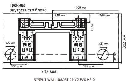
SYSPLIT WALL SMART 09 V2 EVO HP Q
