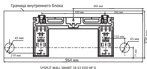
SYSPLIT WALL SMART 18 V2 EVO HP Q
