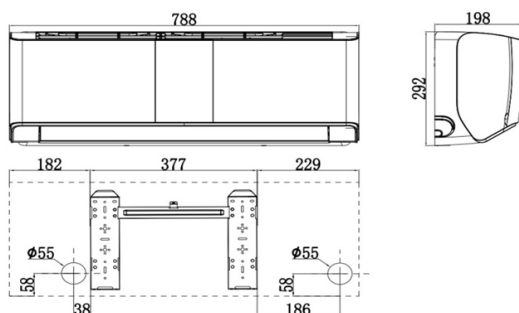
SYSPLIT WALL SIMPLE 07-12 HP Q
