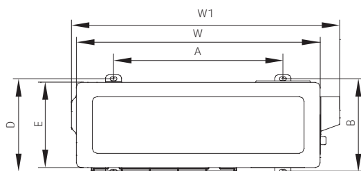
SYSPLIT OUTDOOR 12-36 HP Q/R
