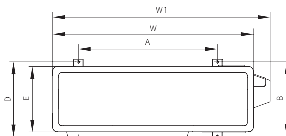
SYSPLIT OUTDOOR 48, 60 HP R
