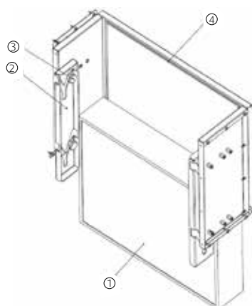
Figure 13.3-2 - Filter Replacement
