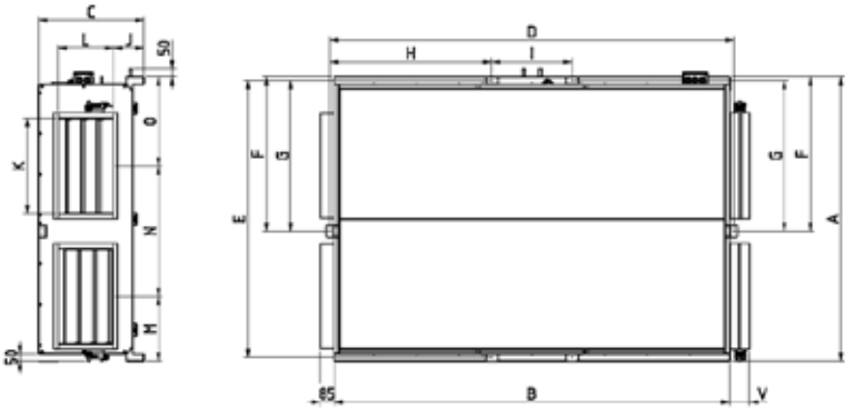
Figure 7.1-1 -Unit Dimensions
