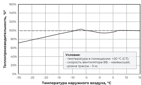
RCI-FHE75HN/OUT
