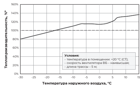
RCI-FHE28HN/OUT
