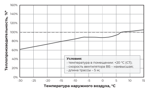
RCI-FHE40HN/OUT
