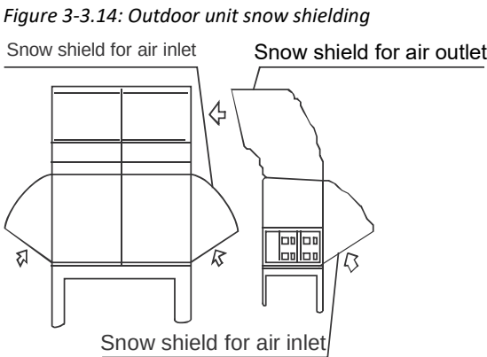
Figure 3-3.14: Outdoor unit snow shielding
