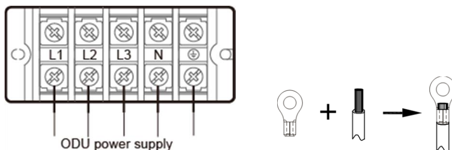
Figure 3-8.2: Outdoor unit 3-phase power supply terminals
