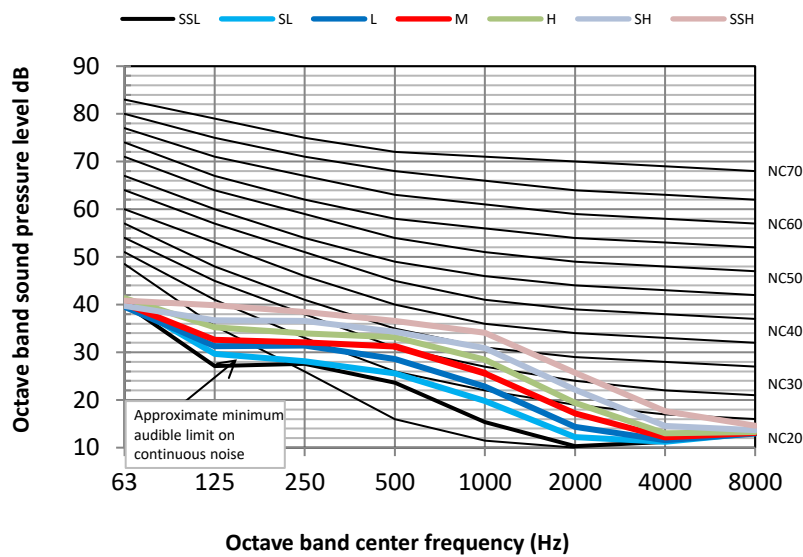
Figure 9.8: MVM71TA-VA1 octave band levels
