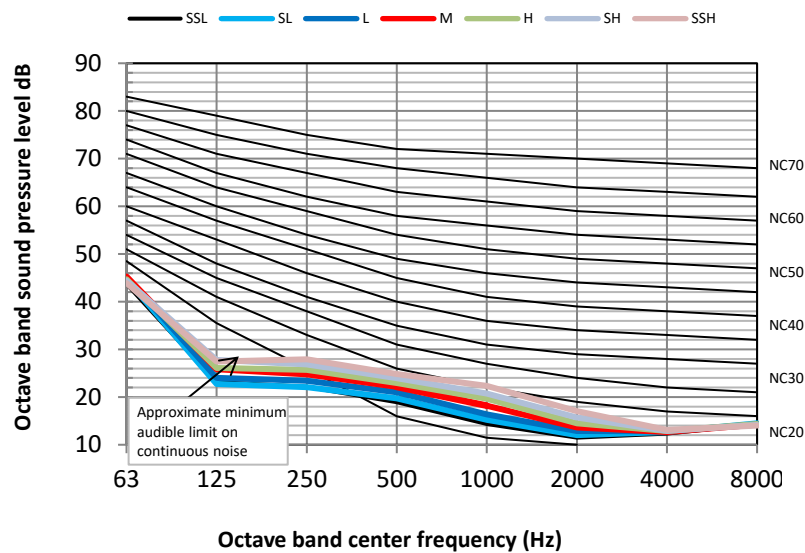
Figure 9.3: MVM22TA-VA1 octave band levels
