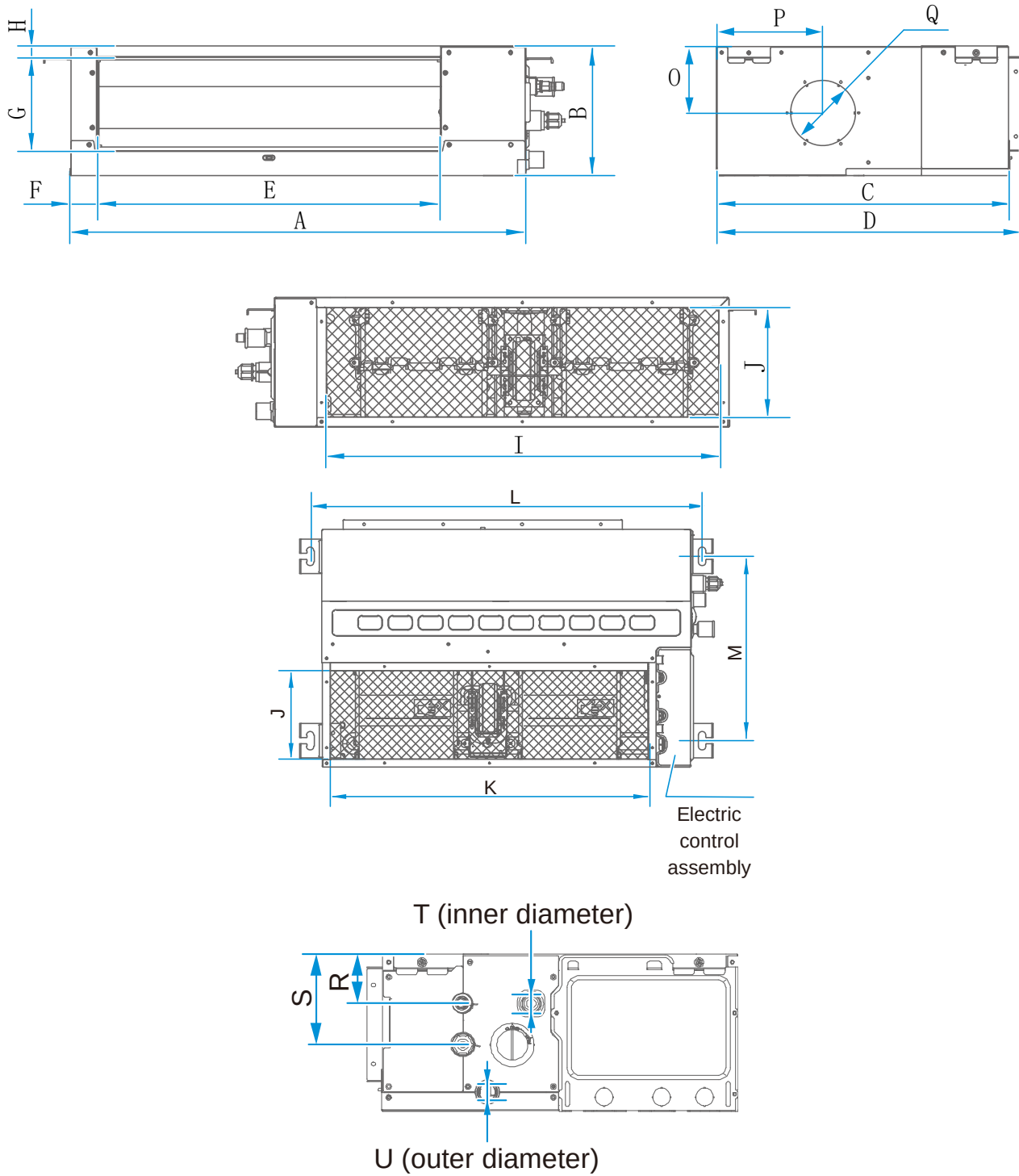
Figure 2.1: External dimensions and size of air outlet opening
