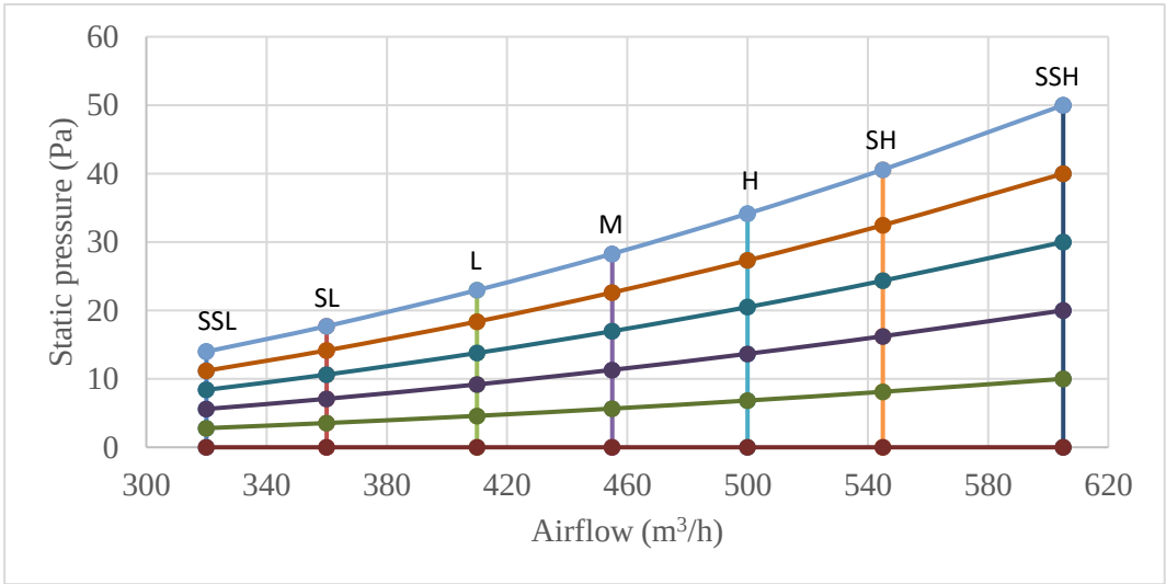
Figure 6.4: MVM36TA-VA1(At) fan performance
