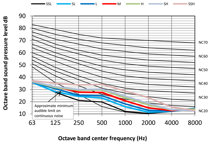
Figure 9.6: MVM45TA-VA1 octave band levels
