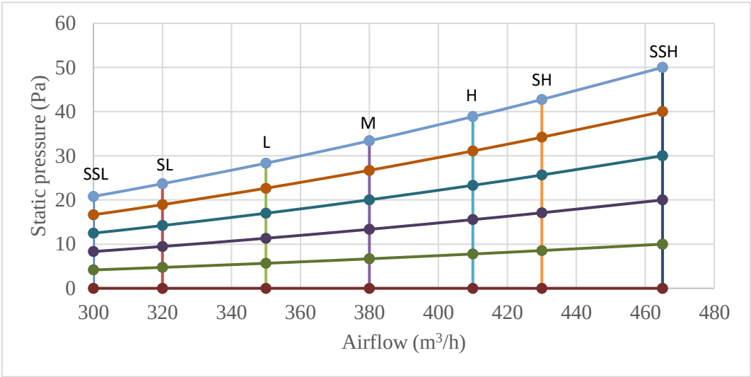
Figure 6.3: MVM28TA-VA1(At) fan performance
