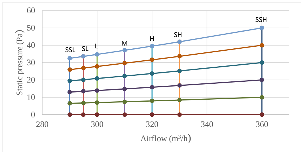
Figure 6.1: MVM15TA-VA1 (At) fan performance
