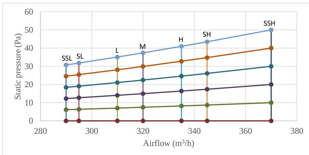
Figure 6.2: MVM22TA-VA1(At) fan performance
