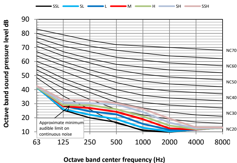
Figure 9.5: MVM36TA-VA1 octave band levels
