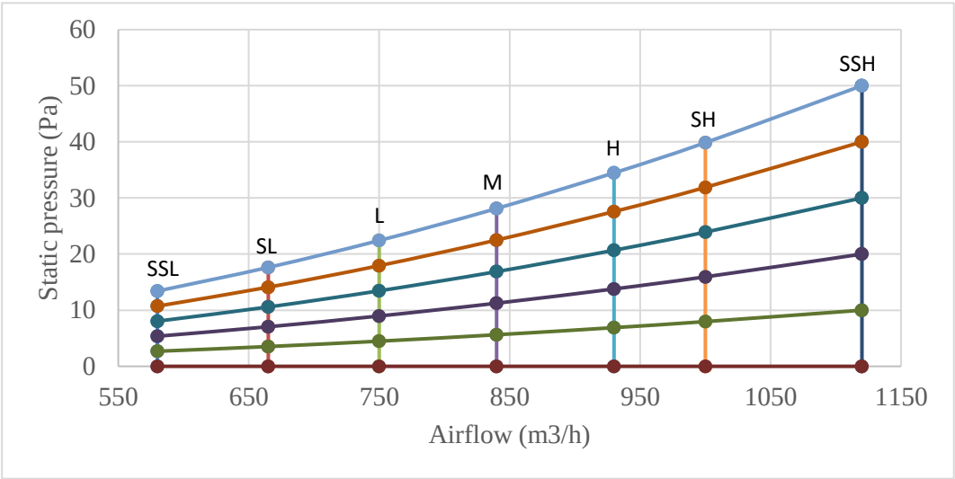
Figure 6.7: MVM71TA-VA1(At) fan performance
