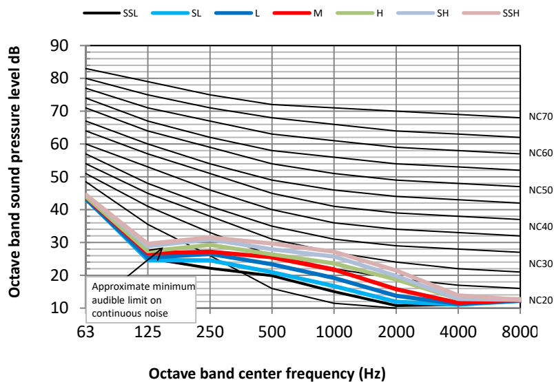
Figure 9.4: MVM28TA-VA1 octave band levels
