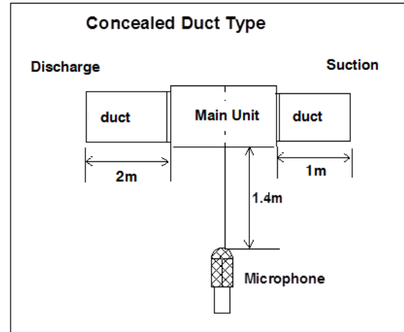
Figure 9.1: Arc series duct sound pressure level measurement
