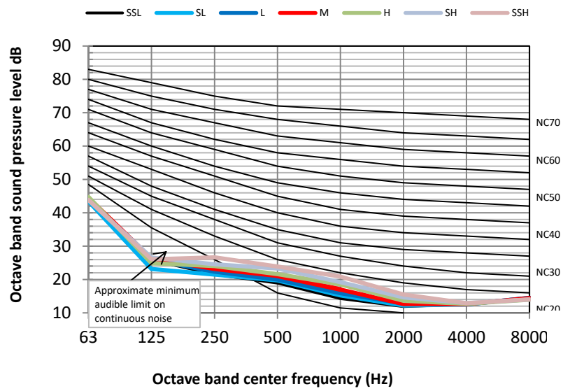
Figure 9.2: MVM15TA-VA1 octave band levels
