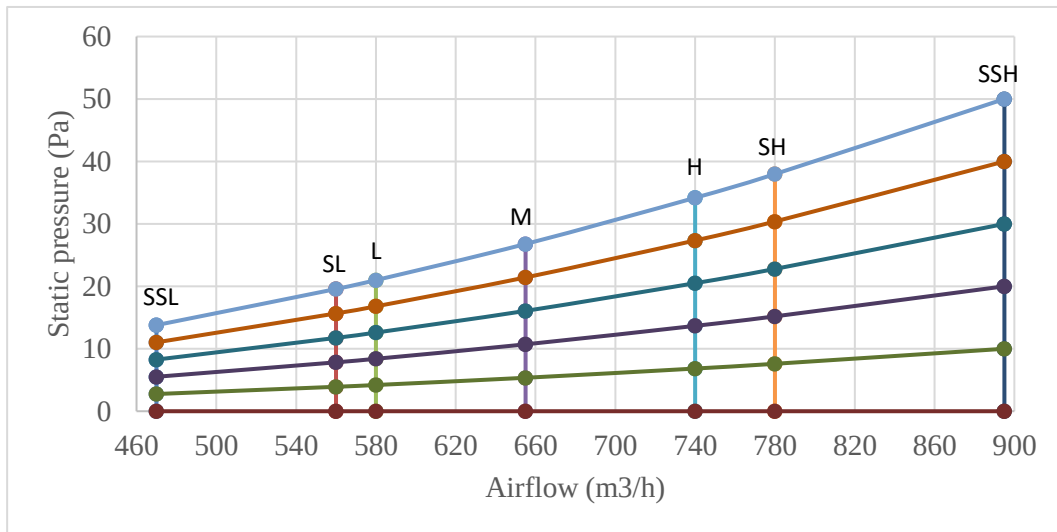
Figure 6.6: MVM56TA-VA1(At) fan performance
