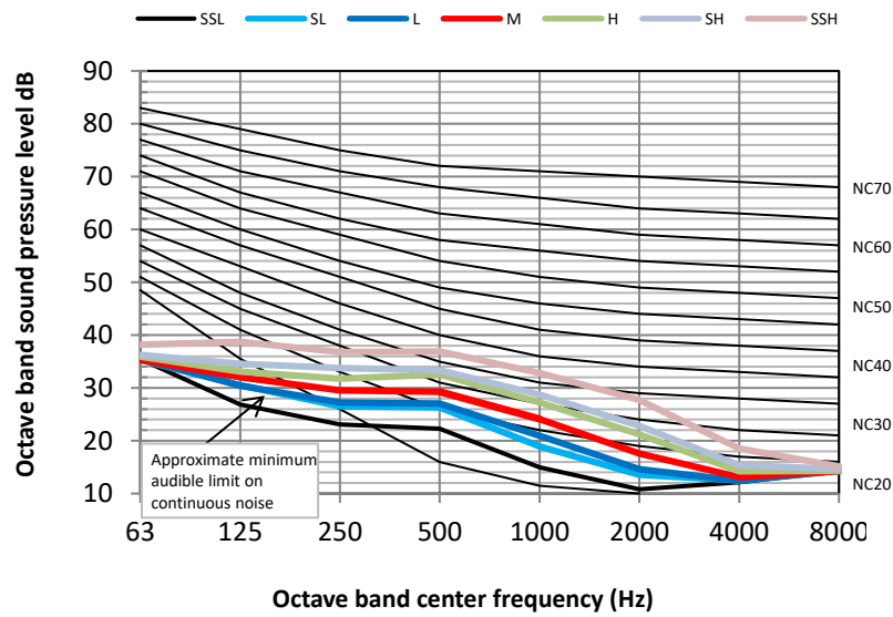
Figure 9.7: MVM56TA-VA1) octave band levels
