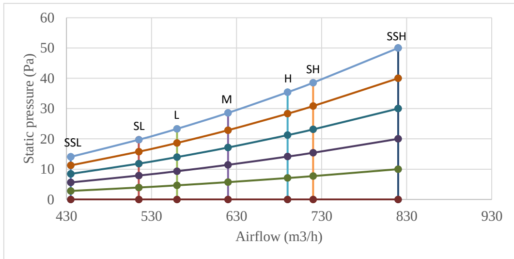
Figure 6.5: MVM45TA-VA1 (At) fan performance
