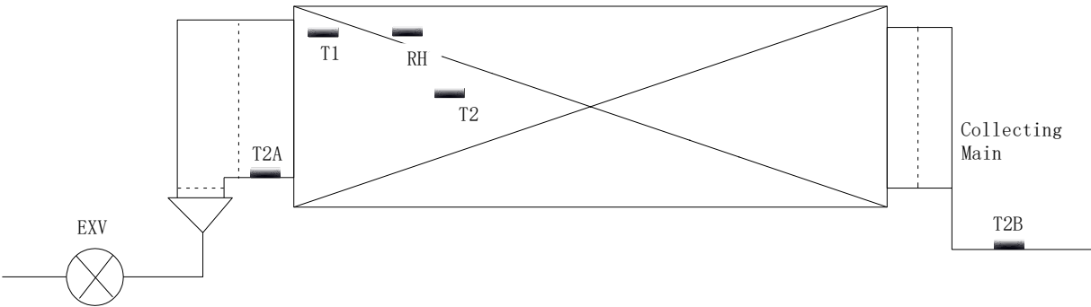
Figure 4.1: Arc series Duct piping diagram
