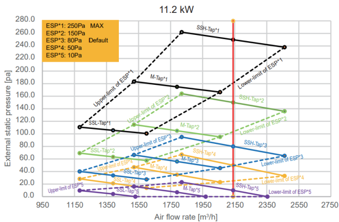
Figure 9.13: MIH112T1HN18
