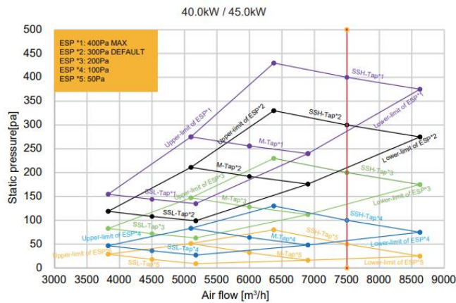
Figure 9.19: MIH400(450)T1HN18
