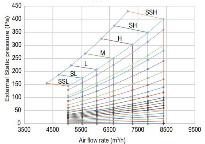
Figure 9.10: MIH560T1HN18
