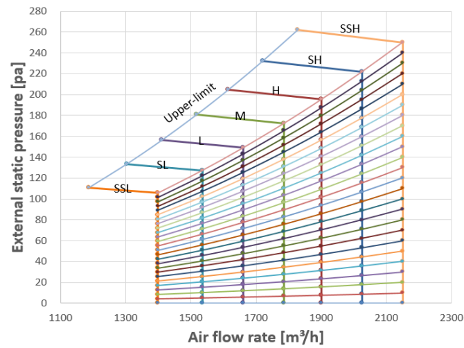
Figure 9.6: MIH160T1HN18
