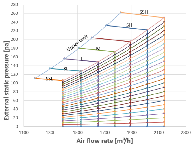
Figure 9.5: MIH140T1HN18
