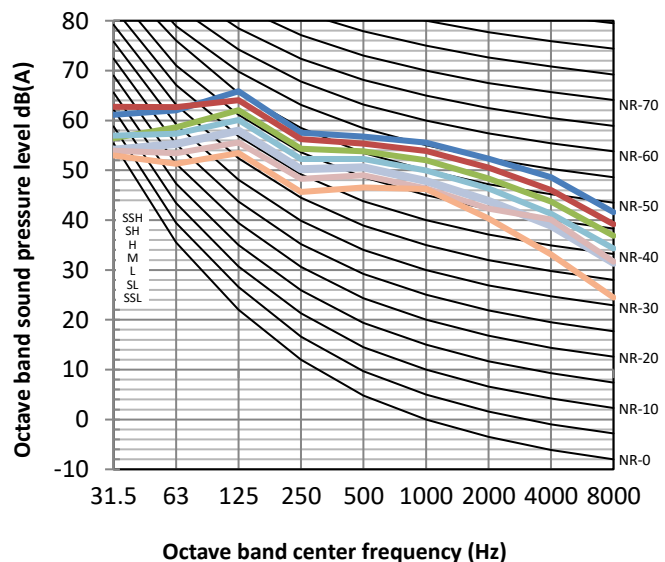
Figure 8.15: MIH560T1HN18 octave band levels
