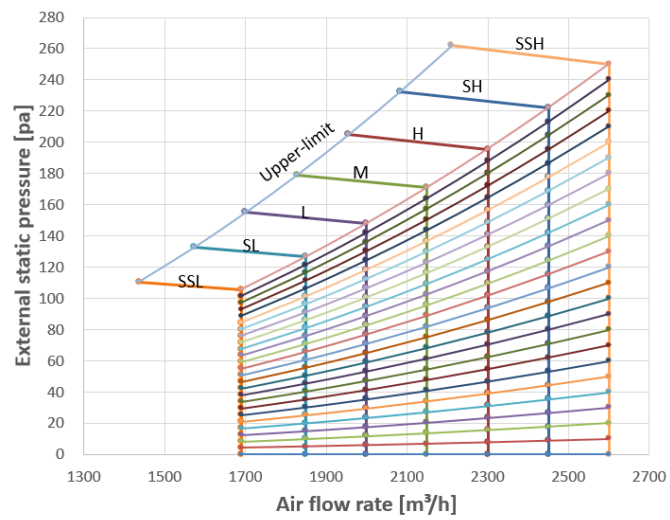
Figure 9.8: MIH335T1HN18
