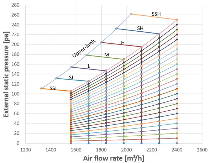
Figure 9.7: MIH200(224,252,280)T1HN18
