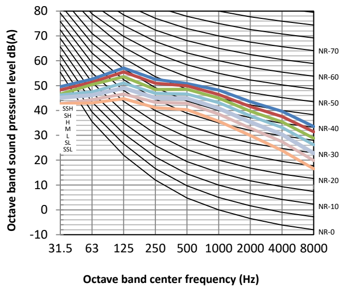
Figure 8.11: MIH280T1HN18 octave band levels
