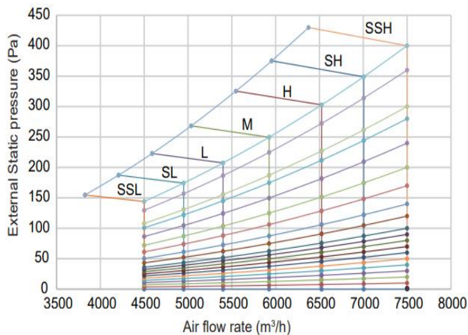
Figure 9.9: MIH400(450)T1HN18
