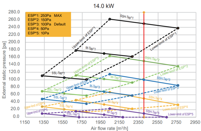
Figure 9.15: MIH140T1HN18
