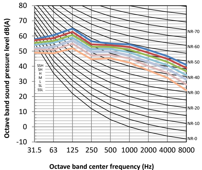
Figure 8.13: MIH400T1HN18 octave band levels
