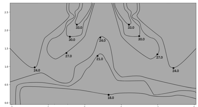
Figure 9.2: MIH15Q4CHN18 heating at 300s
