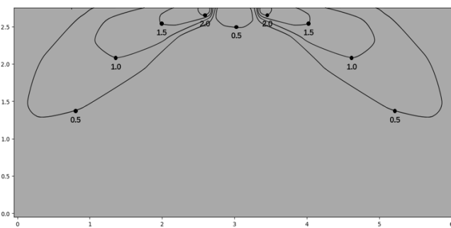
Figure 9.5: MIH28Q4CHN18 cooling at 300s
