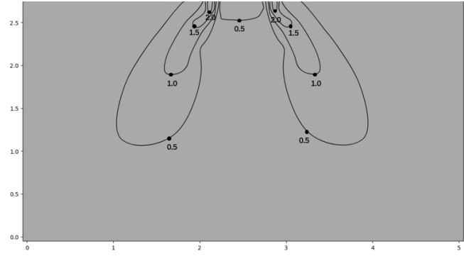
Figure 9.4: MIH22Q4CHN18 heating at 300s
