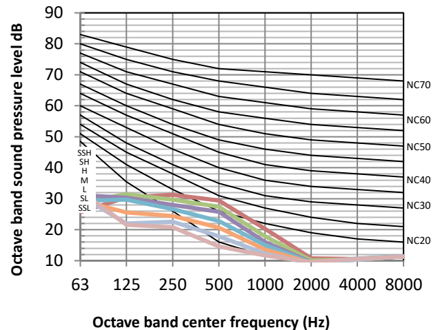
Figure 8.3: MIH36Q4CHN18 octave band levels
