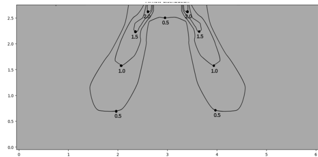
Figure 9.6: MIH28Q4CHN18 heating at 300s
