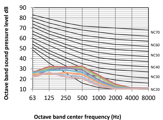
Figure 8.3: MIH36Q4CHN18 octave band levels
