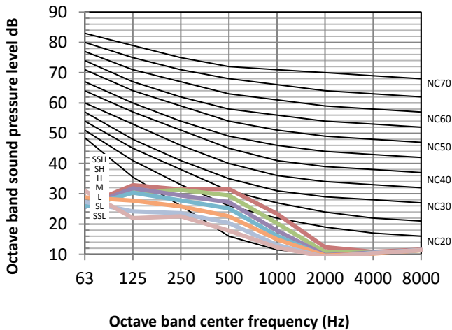
Figure 8.2: MIH28Q4CHN18 octave band levels
