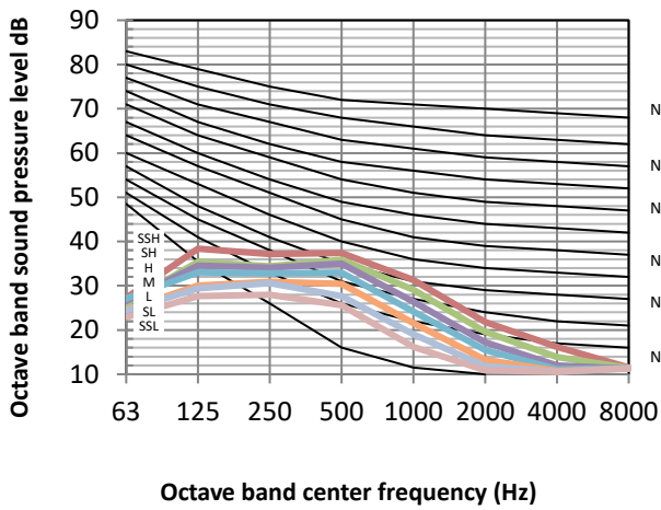
Figure 8.2: MIH63Q4CHN18 octave band levels
