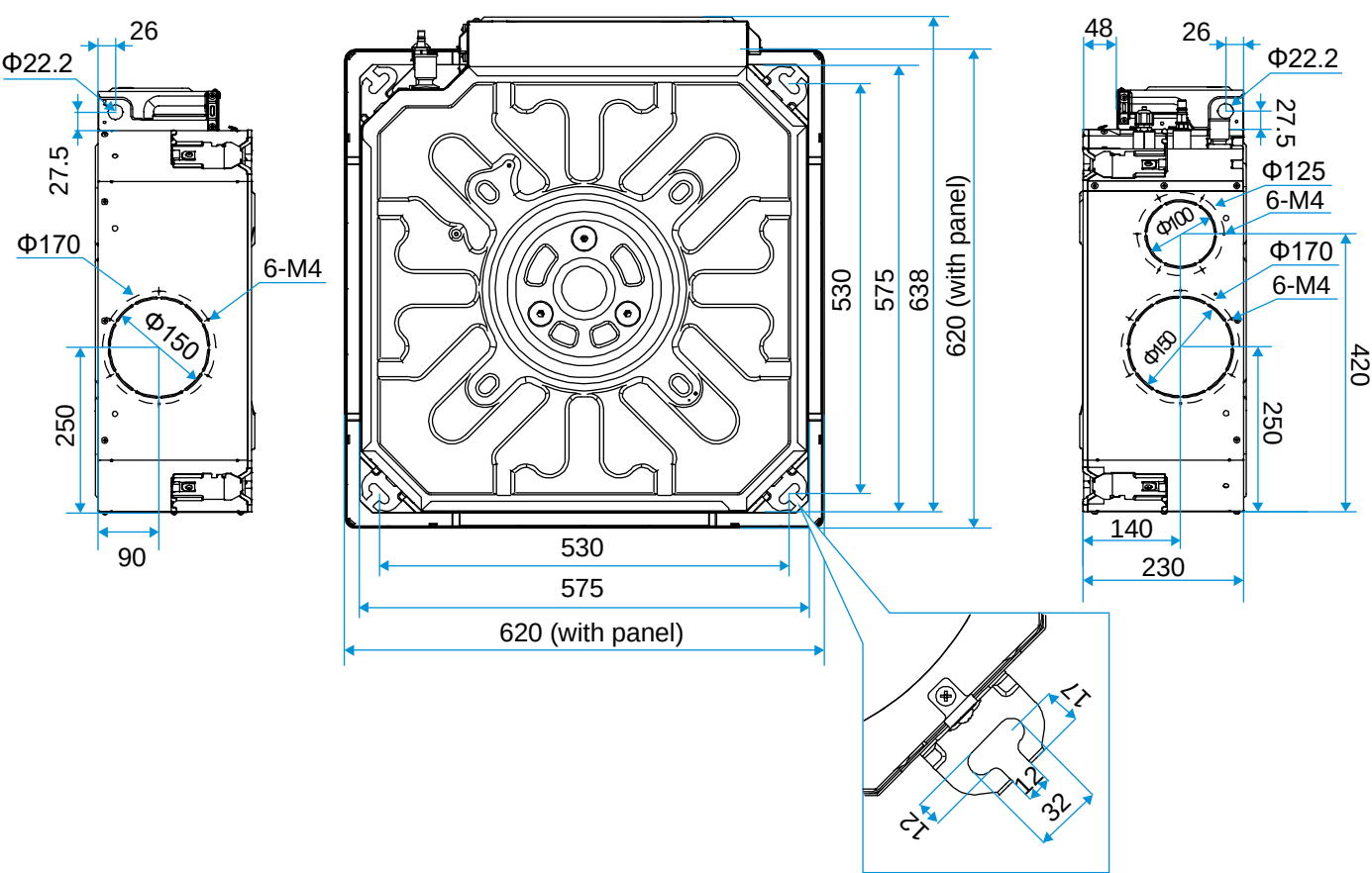
Figure 2.1: Compact Four-way Cassette dimensions (unit: mm)
