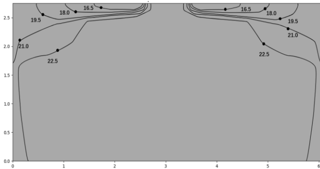
Figure 9.25: MIH45Q4HN18 cooling at 300s
