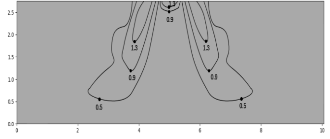
Figure 9.20: MIH140Q4HN18 heating at 300s
