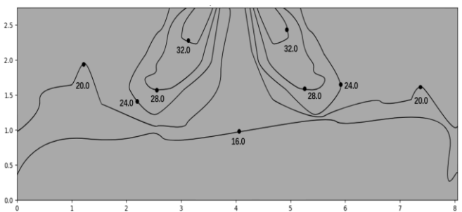
Figure 9.30: MIH71Q4HN18 heating at 300s
