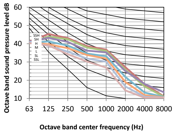
Figure 8.11: MIH140Q4HN18 octave band levels
