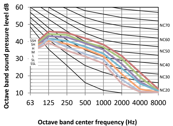
Figure 8.3: MIH36Q4HN18 octave band levels
