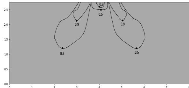
Figure 9.14: MIH90Q4HN18 heating at 300s
