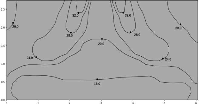
Figure 9.26: MIH45Q4HN18 heating at 300s
