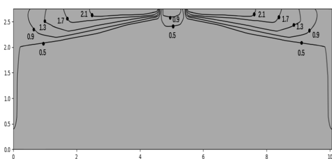
Figure 9.15: MIH100Q4HN18 cooling at 300s
