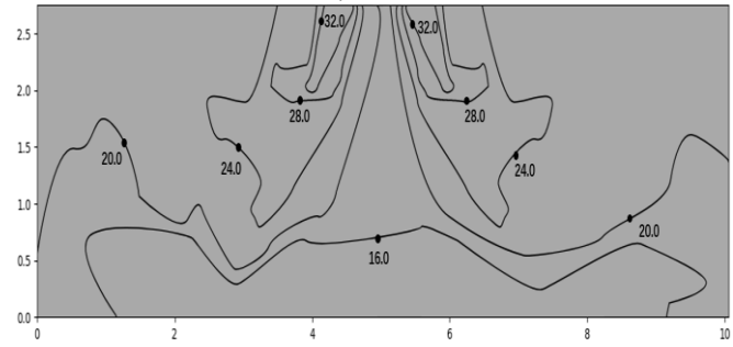
Figure 9.36: MIH100Q4HN18 heating at 300s
