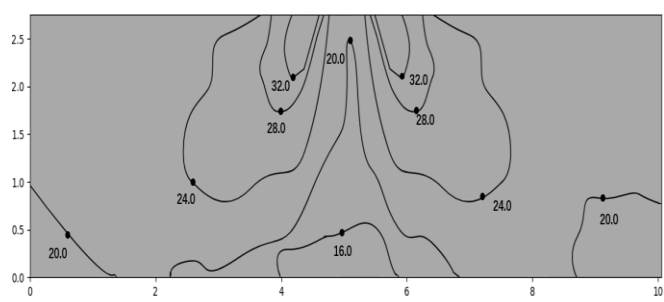
Figure 9.40: MIH180Q4HN18 heating at 300s
