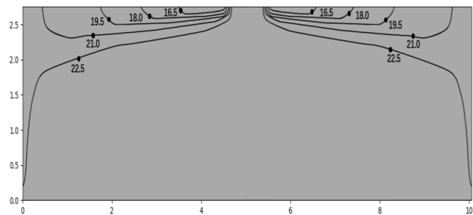
Figure 9.39: MIH180Q4HN18 cooling at 300s
