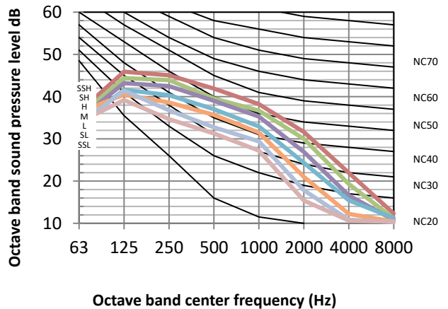
Figure 8.3: MIH36Q4HN18 octave band levels
