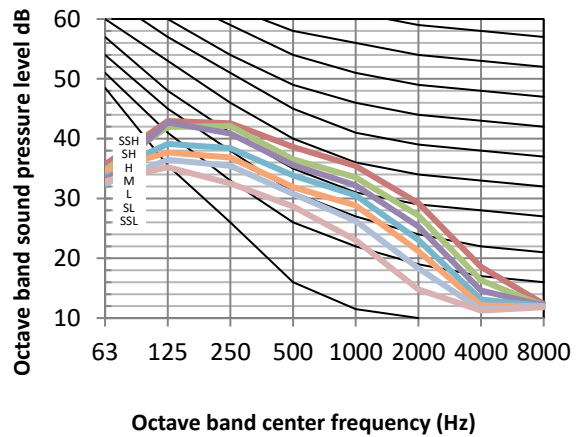
Figure 8.9: MIH100Q4HN18 octave band levels
