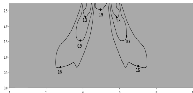
Figure 9.16: MIH100Q4HN18 heating at 300s
