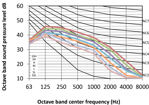
Figure 8.2: MIH28Q4HN18 octave band levels
