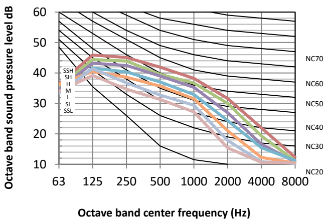
Figure 8.2: MIH28Q4HN18 octave band levels
