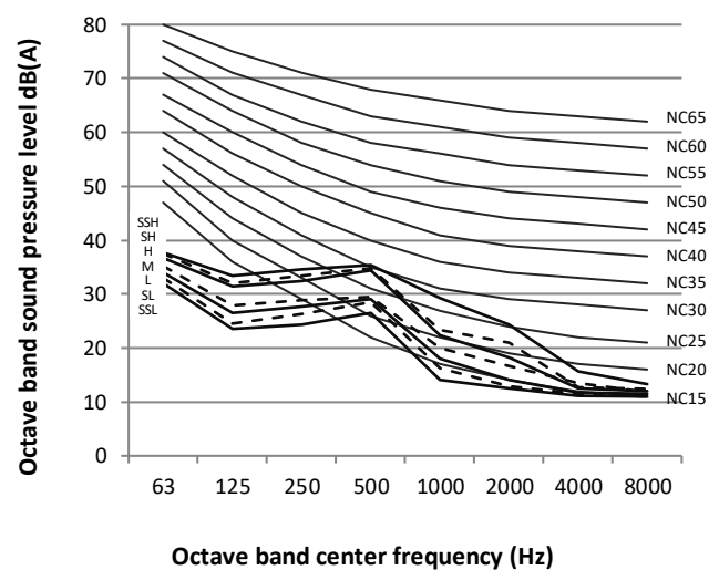
Figure 8.3: MIH36Q2HN18 octave band levels
