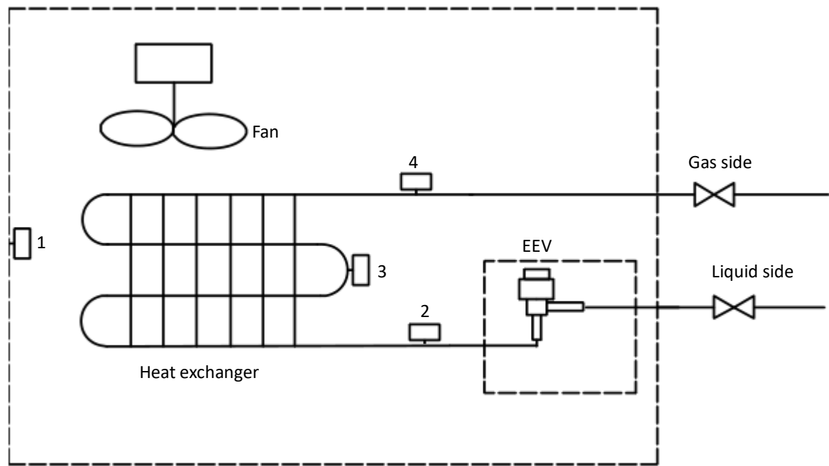
Figure 4.1: Two-way Cassette piping diagram
