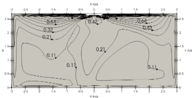
Figure 9.5: MIH36Q2HN18 cooling at 300S
