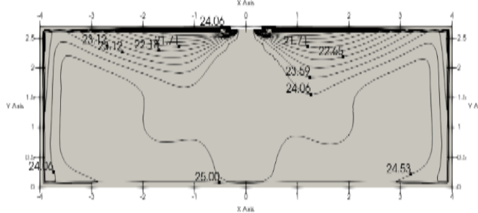
Figure 9.19: MIH45Q2HN18 cooling at 300S
