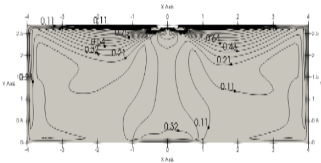
Figure 9.7: MIH45Q2HN18 cooling at 300S
