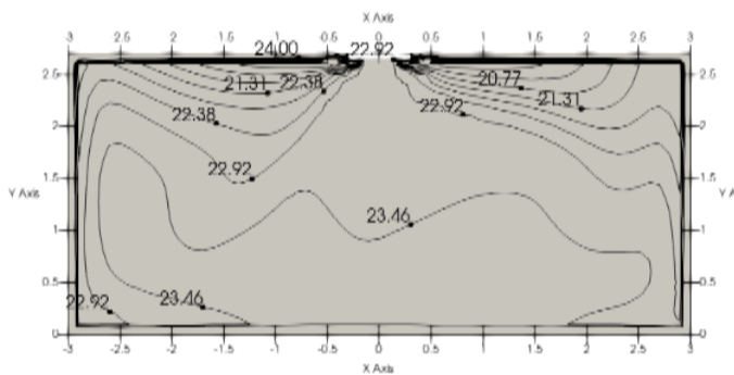
Figure 9.17: MIH36Q2HN18 cooling at 300S
