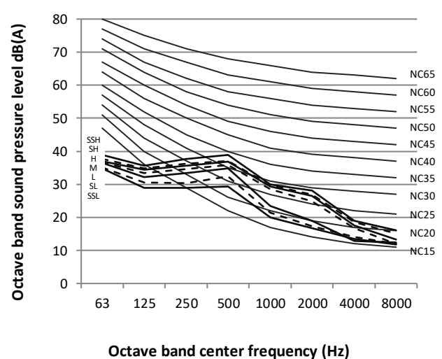
Figure 8.5: MIH56Q2HN18 octave band levels
