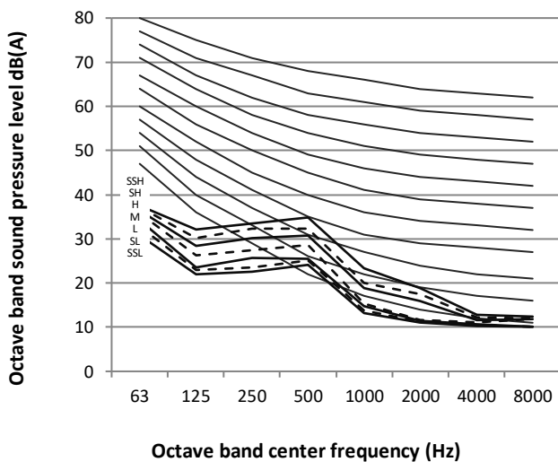
Figure 8.2: MIH22(28)Q2HN18 octave band levels
