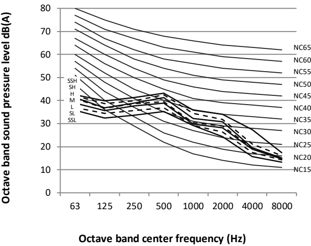
Figure 8.6: MIH71Q2HN18 octave band levels
