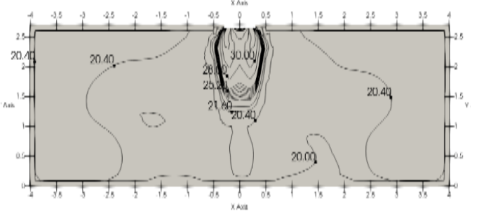
Figure 9.20: MIH45Q2HN18 heating at 300S
