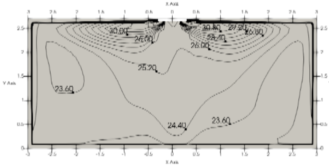
Figure 9.22: MIH56Q2HN18 heating at 300S
