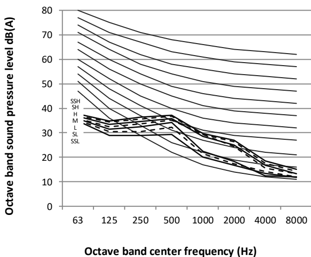
Figure 8.4: MIH45Q2HN18 octave band levels
