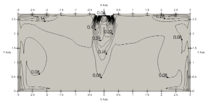
Figure 9.6: MIH36Q2HN18 heating at 300S
