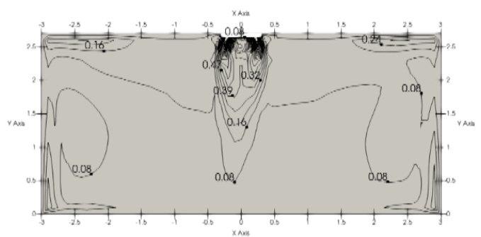
Figure 9.4: MIH28Q2HN18 heating at 300S
