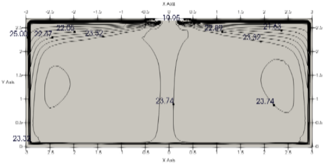
Figure 9.21: MIH56Q2HN18 cooling at 300S
