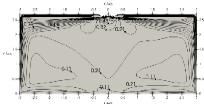
Figure 9.9: MIH56Q2HN18 cooling at 300S
