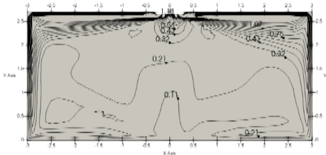
Figure 9.11: MIH71Q2HN18 cooling at 300S
