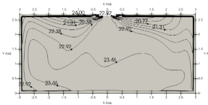
Figure 9.15: MIH28Q2HN18 cooling at 300S
