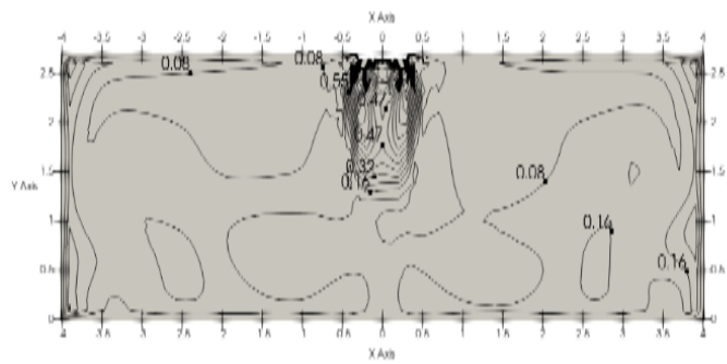
Figure 9.8: MIH45Q2HN18 heating at 300S
