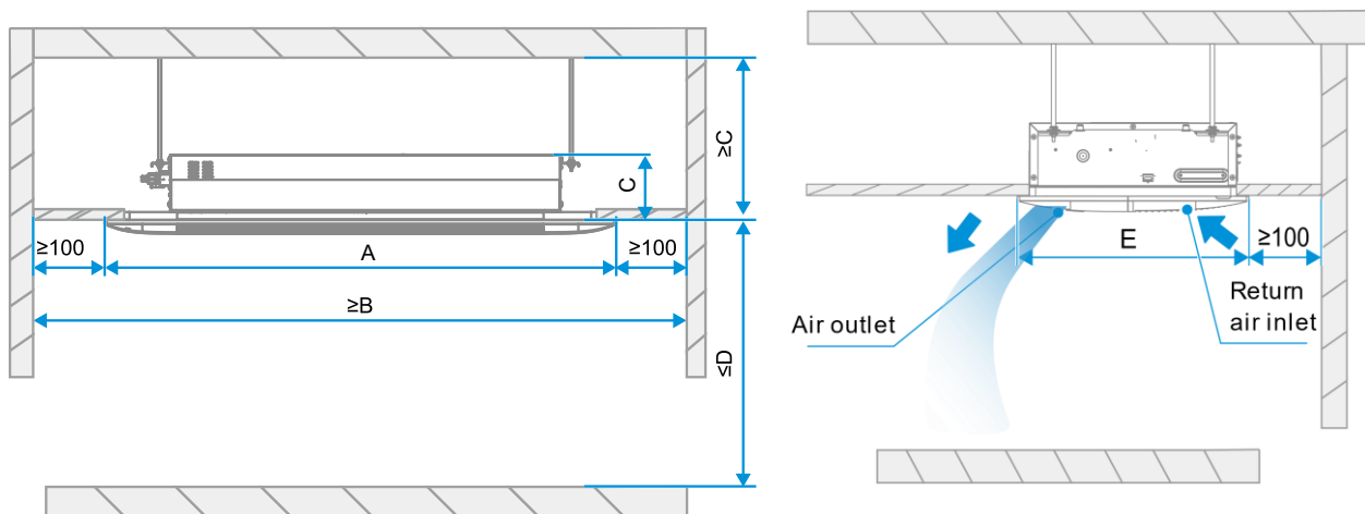
Figure 3.1: One-way Cassette space requirements (unit: mm)
