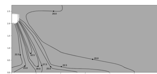
Figure 9.26: MIH45GHN18 heating at 300S
