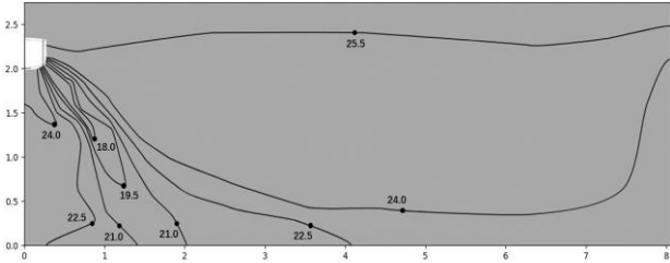
Figure 9.29: MIH71GHN18 cooling at 300S
