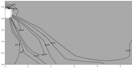
Figure 9.9: MIH45GHN18 cooling at 300S
