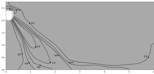
Figure 9.11: MIH56GHN18 cooling at 300S
