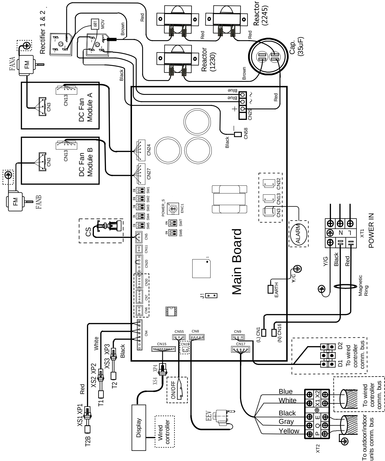
Figure 5.4: MI2-400(450,560)T1DHN1 wiring diagram
