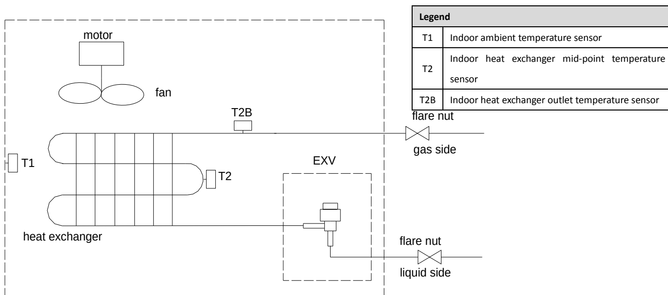
Figure 4.1: MI2-71(80,90,112,140,160,200,250,280,400,450,560)T1DHN1 piping diagram
