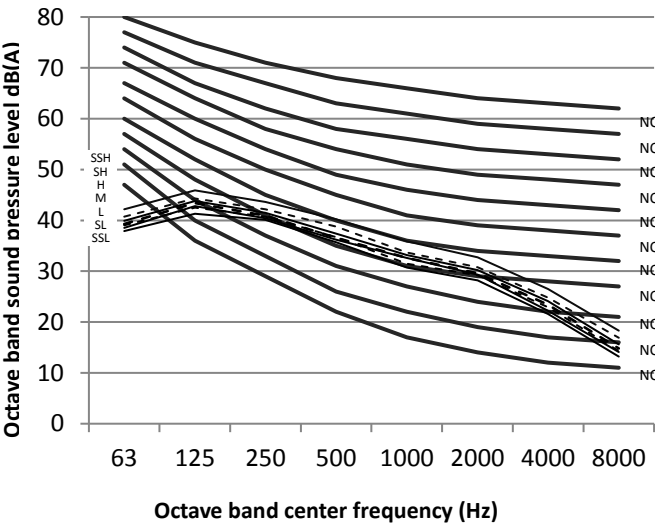
Figure 9.2: MI2-71(80)T1DHN1 octave band levels
