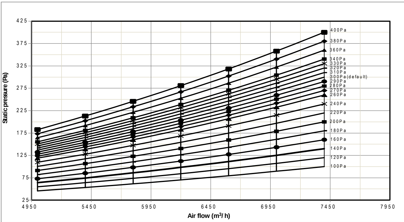
Figure 6.8: MI2-560T1DHN1 fan performance
