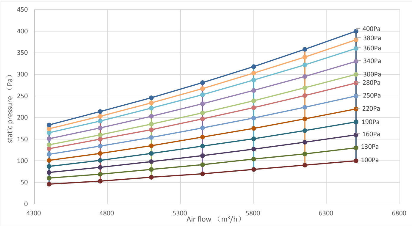
Figure 6.7: MI2-400(450)T1DHN1 fan performance
