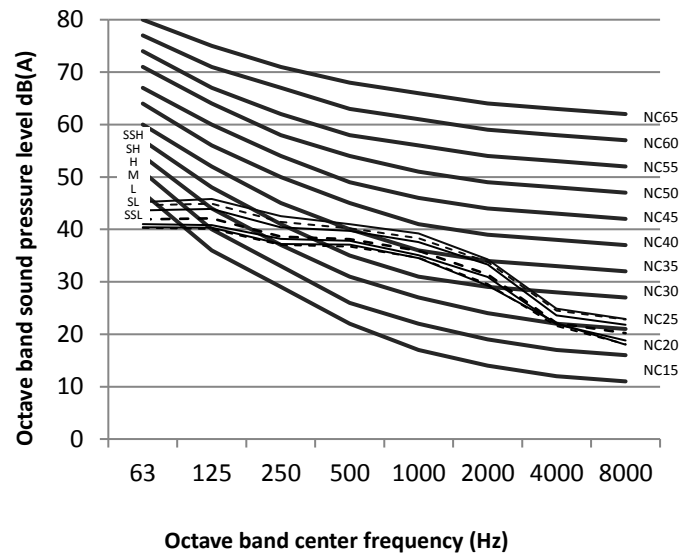
Figure 9.7: MI2-200(250,280)T1DHN1 octave band levels
