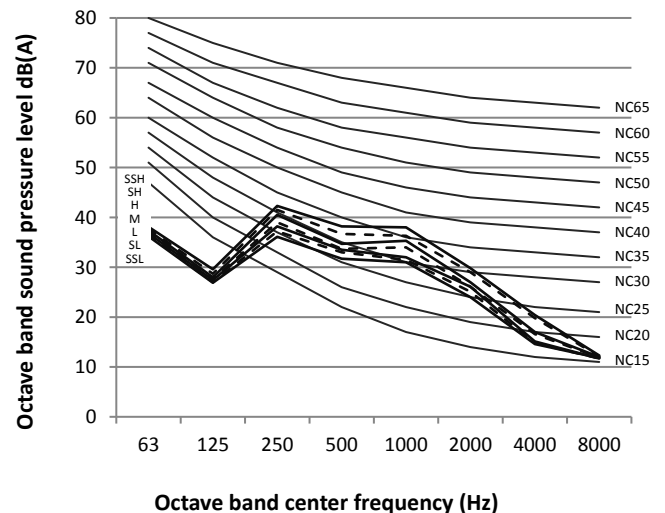
Figure 8.5: MI2-45Q1DHN1 octave band levels
