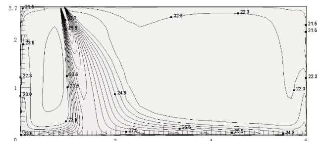
Figure 9.22: MI2-36Q1DHN1 heating at 300S
