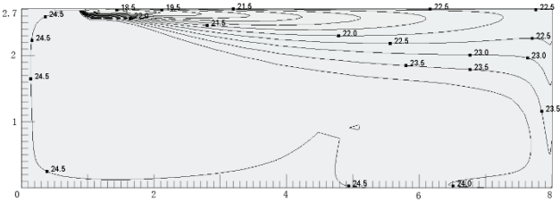
Figure 9.25: MI2-56Q1DHN1 cooling at 300S
