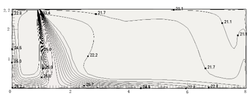
Figure 9.26: MI2-56Q1DHN1 heating at 300S
