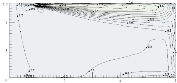
Figure 9.7: MI2-36Q1DHN1 cooling at 300S
