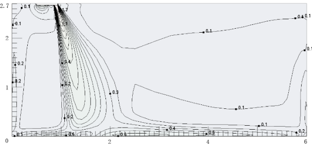
Figure 9.8: MI2-36Q1DHN1 heating at 300S
