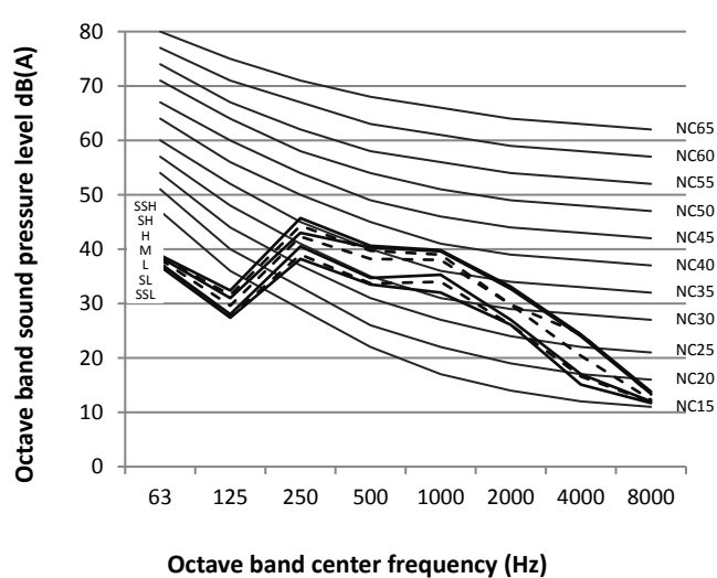
Figure 8.7: MI2-71Q1DHN1 octave band levels
