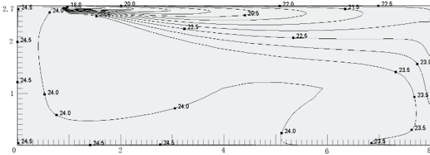
Figure 9.27: MI2-71Q1DHN1 cooling at 300S
