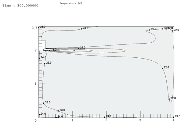
Figure 9.21: MI2-22GDN1 cooling at 300S
