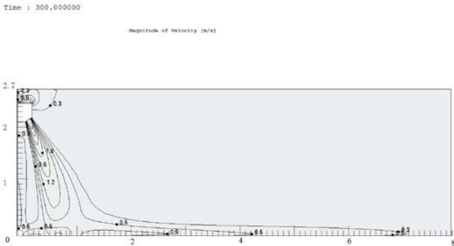
Figure 9.14: MI2-71GDN1 heating at 300S
