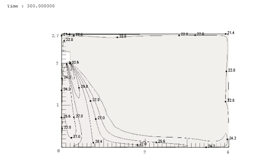
Figure 9.20: MI2-17GDN1 heating at 300S
