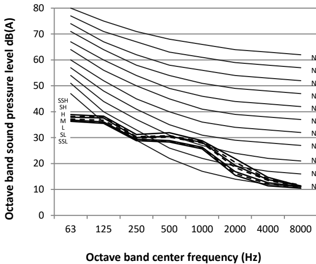
Figure 8.6: MI2-71(80)GDN1 octave band levels
