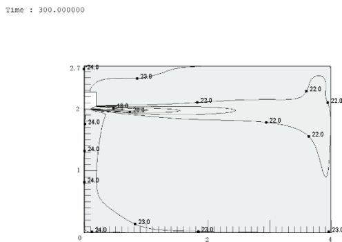
Figure 9.21: MI2-22GDN1 cooling at 300S
