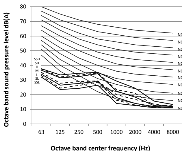
Figure 8.5: MI2-160DLHDN1 octave band levels
