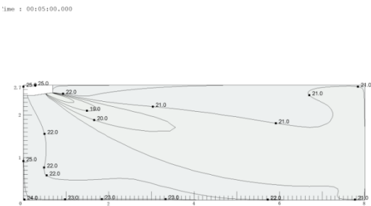
Figure 9.31: MI2-160DL DHN1 cooling at 300S
