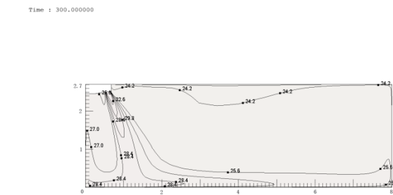
Figure 9.32: MI2-160DL DHN1 heating at 300S
