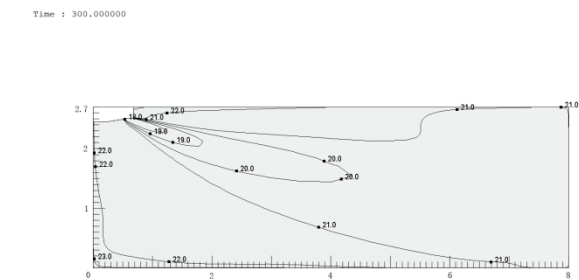
Figure 9.31: MI2-160DL DHN1 cooling at 300S
