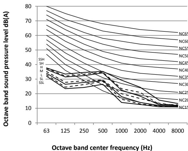
Figure 8.2: MI2-36DLHDN1 octave band levels
