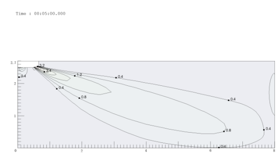
Figure 9.11: MI2-90DLHDN1 cooling at 300S
