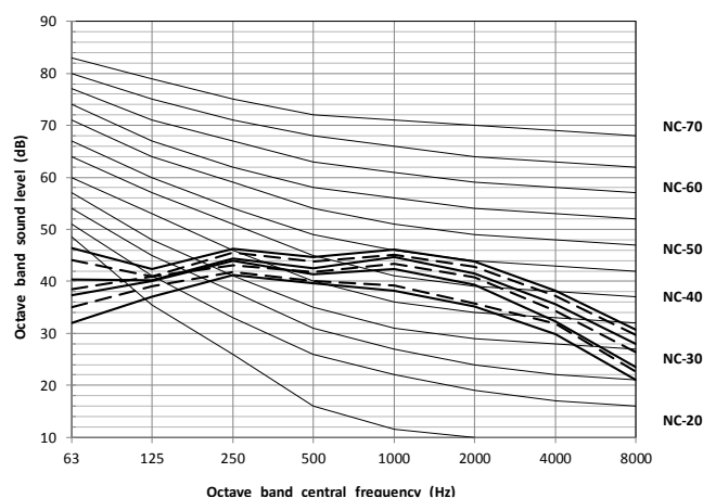
Figure 8.5: MI2-160DLHDN1 octave band levels
