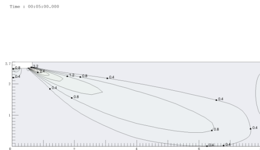
Figure 9.7: MI2-71DL DHN1 cooling at 300S
