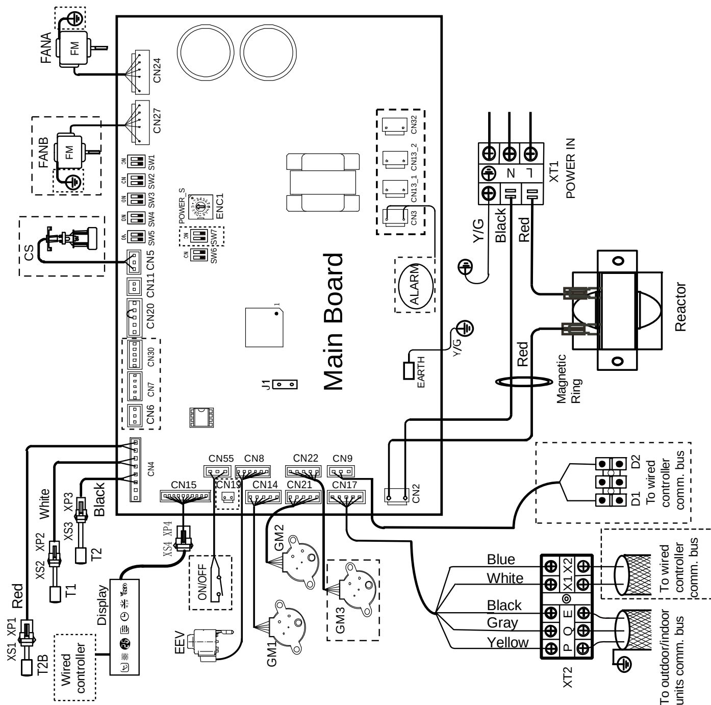
Figure 5.1: Ceiling & floor MI2-36(45,56,71,80,90,112,140)DL DHN1wiring diagram
