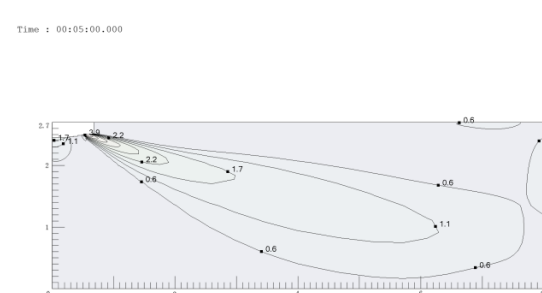
Figure 9.15: MI2-160DLHDN1 cooling at 300S
