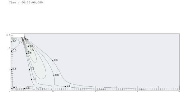
Figure 9.8: MI2-71DL DHN1 heating at 300S
