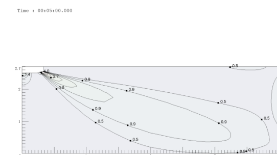
Figure 9.13: MI2-112DLHDN1 cooling at 300S
