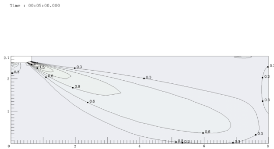
Figure 9.3: MI2-45DL DHN1 cooling at 300S
