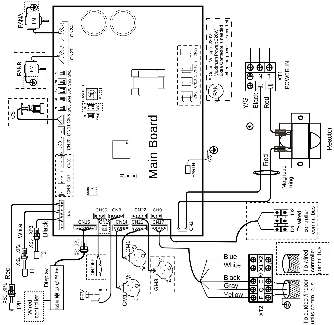
Figure 5.2: Ceiling & floor MI2-160DLDHN1wiring diagram
