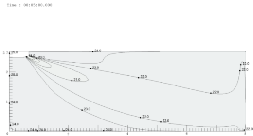
Figure 9.29: MI2-112DL DHN1 cooling at 300S
