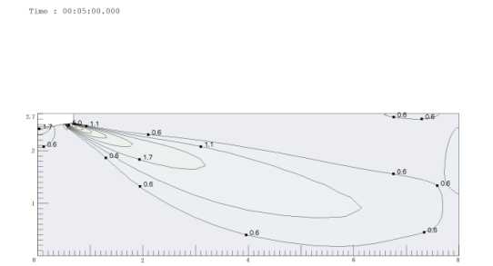
Figure 9.15: MI2-140DLHDN1 cooling at 300S
