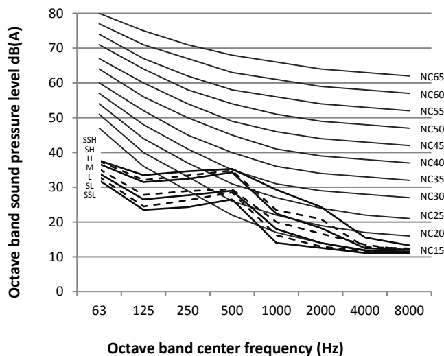
Figure 8.3: MI2-45(56,71)DLHDN1 octave band levels
