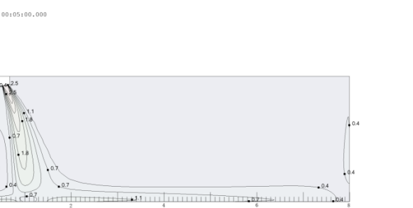
Figure 9.16: MI2-140DLHDN1 heating at 300S
