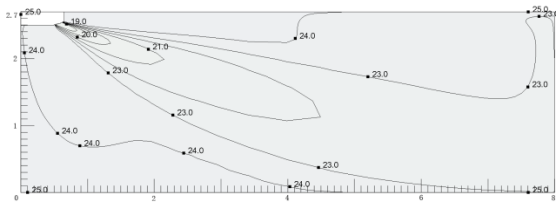
Figure 9.23: MI2-71DLHDN1 cooling at 300S
