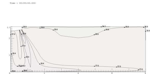
Figure 9.32: MI2-160DL DHN1 heating at 300S
