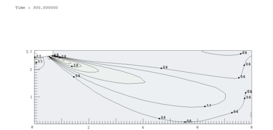
Figure 9.15: MI2-160DLHDN1 cooling at 300S
