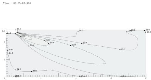
Figure 9.27: MI2-90DL DHN1 cooling at 300S
