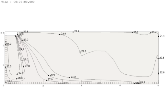
Figure 9.30: MI2-112DL DHN1 heating at 300S
