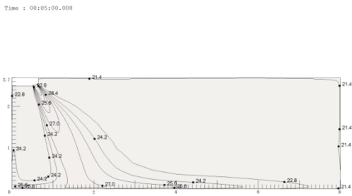
Figure 9.28: MI2-90DL DHN1 heating at 300S
