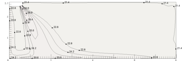
Figure 9.22: MI2-56DLHDN1 heating at 300S
