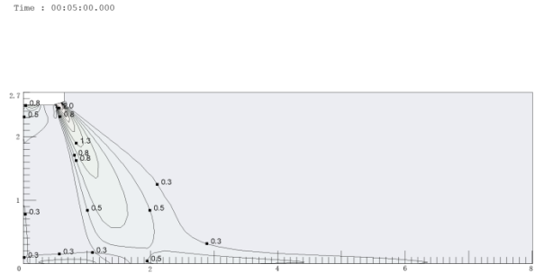
Figure 9.4: MI2-45DL DHN1 heating at 300S
