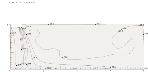
Figure 9.32: MI2-140DL DHN1 heating at 300S
