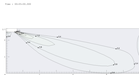
Figure 9.7: MI2-71DL DHN1 cooling at 300S
