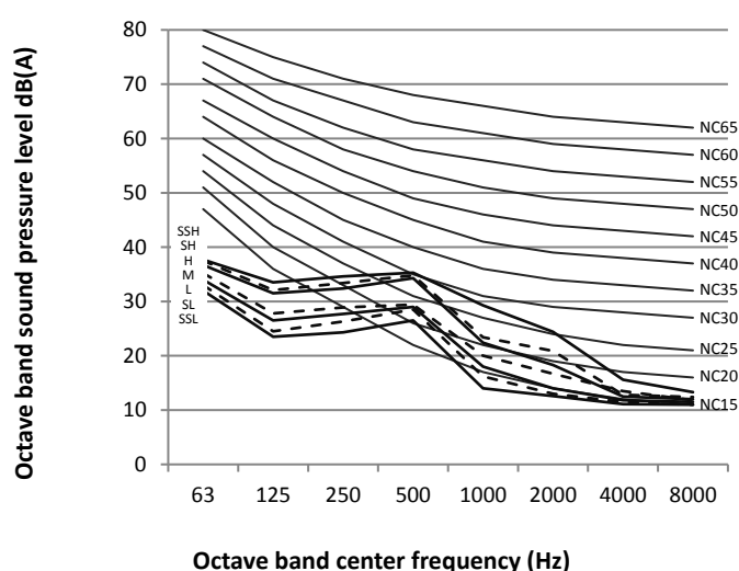
Figure 8.5: MI2-112(140)DLHDN1 octave band levels
