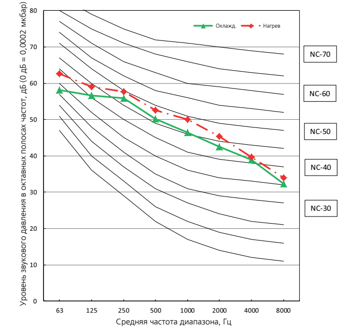
M2OD-18HFN8-Q
