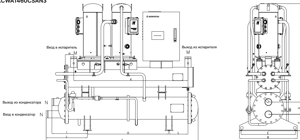
KCWA1460CSAN3
