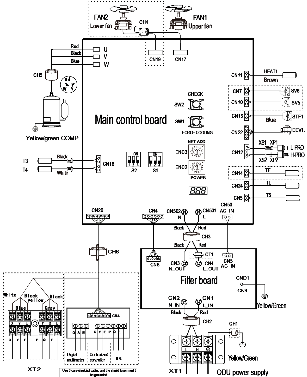
Figure 2-5.3: 140/160 model wiring diagram
