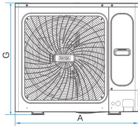
Figure 2-2.3: 100/120 model front view Dimensions (unit: mm)
