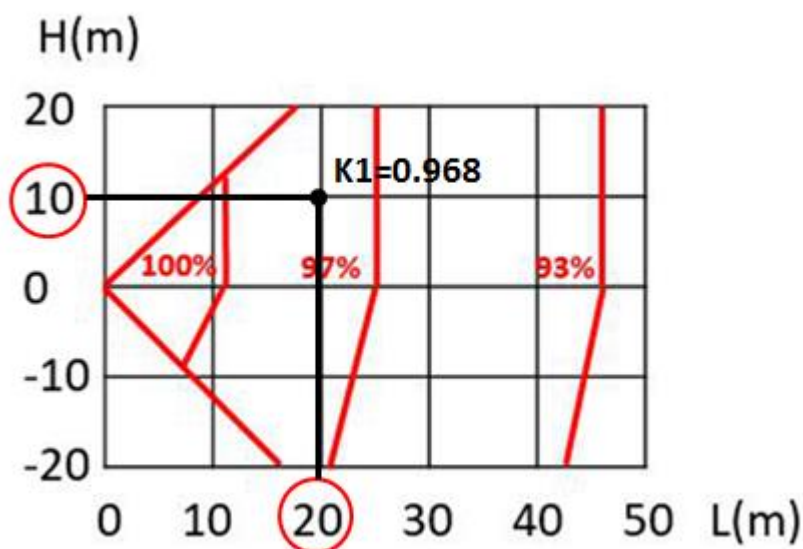
Figure 1-5.3: DX PRO COMPACT rate of change in cooling capacity
