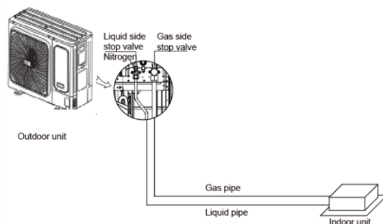
Figure 3-4.11: Gastightness test
