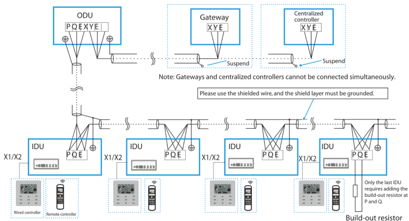
Figure 3-8.4: System communication wiring example
