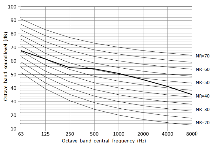
Figure 2-9.3 100 model octave band level
