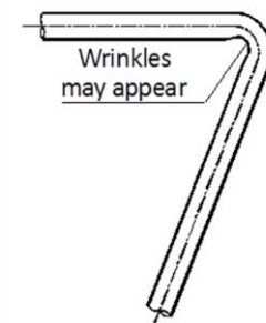
Figure 3-4.3: Pipe bending in excess of 90^\circ
