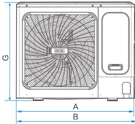
Figure 2-2.5: 140/160 model front view Dimensions (unit: mm)
