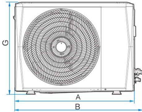
Figure 2-2.1: 80 model front view dimensions (unit: mm)
