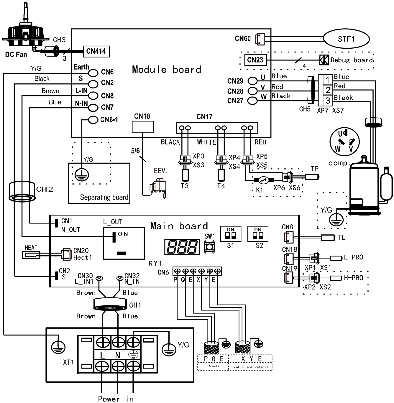
Figure 2-5.1: 80 model wiring diagram
