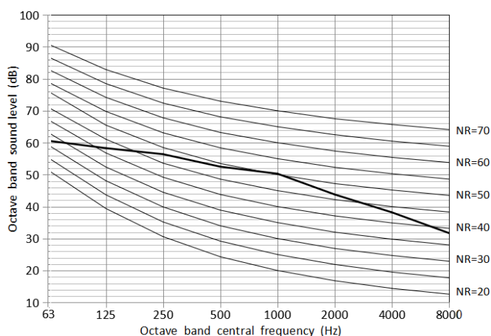
Figure 2-9.2 80 model octave band level
