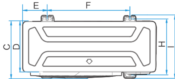
Figure 2-2.4: 140/160 model front top Dimensions (unit: mm)
