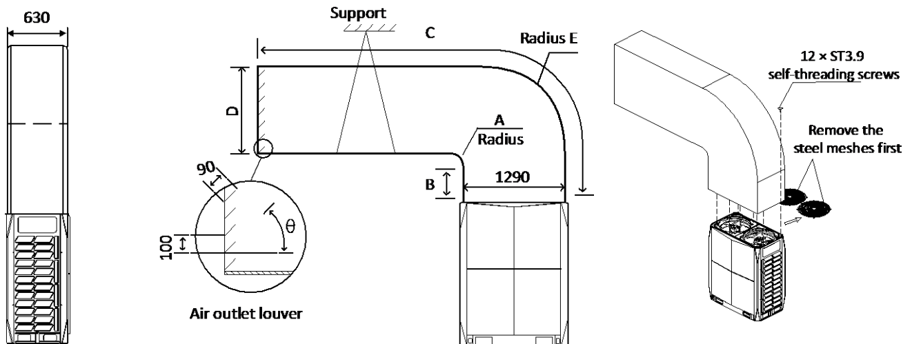
Figure 3-3.7: Longitudinal ducting for 20HP and 22HP units (unit: mm)
