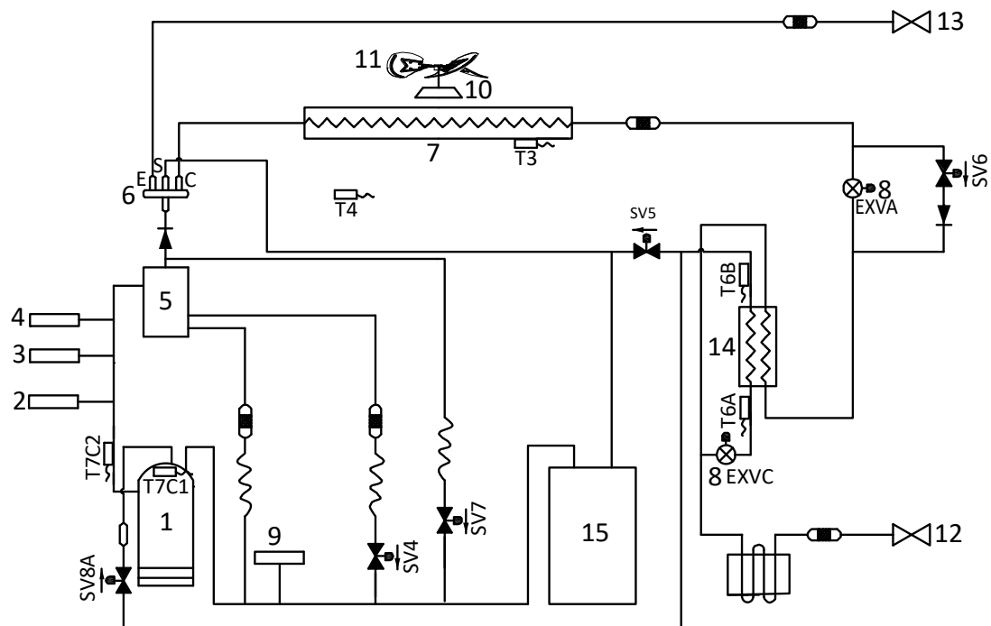
Figure 2-4.2: 14/16/18HP piping diagram
