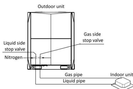
Figure 3-5.11: Gastightness test
