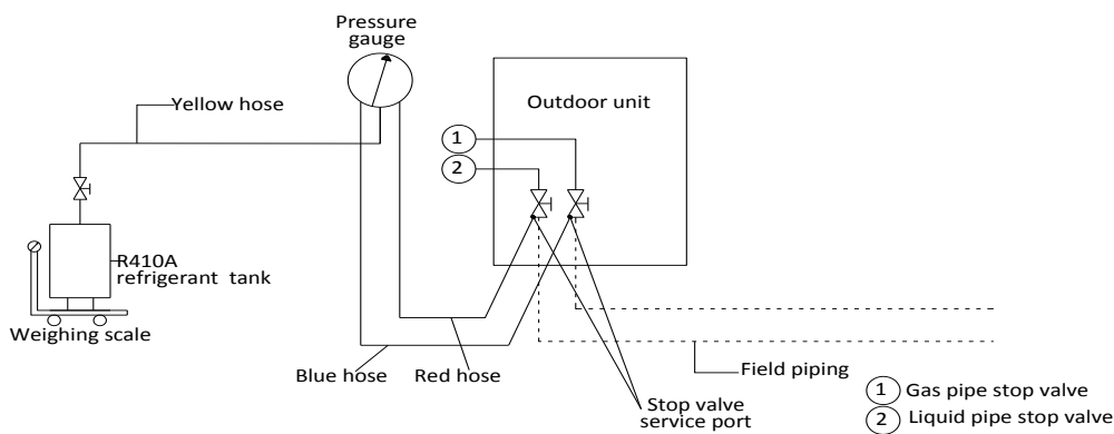
Figure 3-8.1: Charging refrigerant
