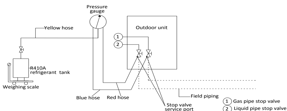
Figure 3-5.12: Vacuum drying
