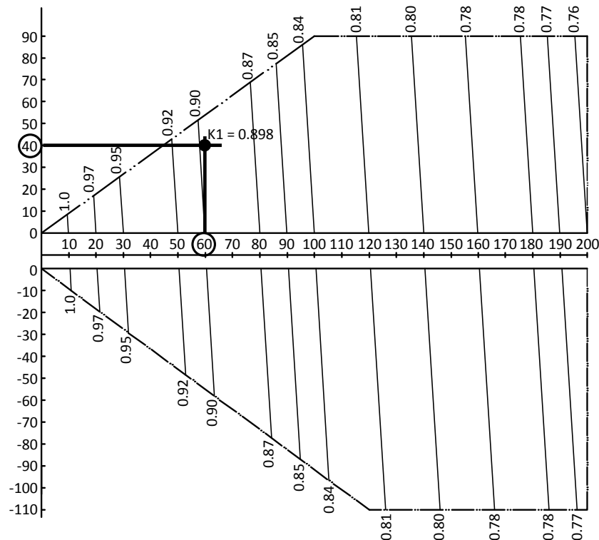
Figure 1-5.3: KTRA-i rate of change in cooling capacity
