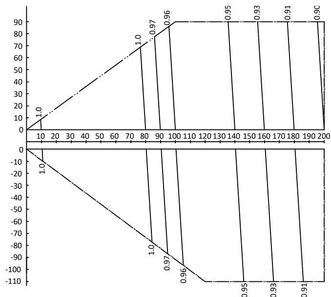
Figure 2-8.2: Rate of change in heating capacity
