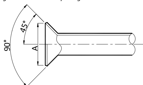
Figure 3-5.2: Flared opening
