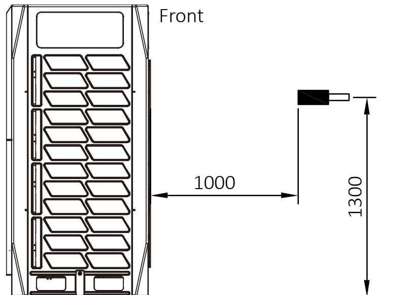
Figure 2-10.1: Sound pressure level measurement (unit: mm)
