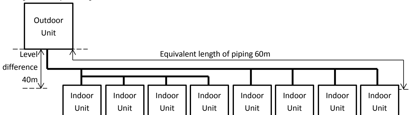
Figure 1-5.2: System diagram
