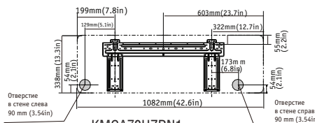
KMGA70HZRN1
