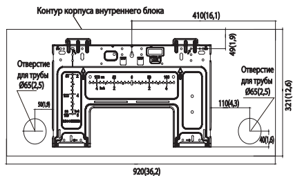
KSGOM26HZRN1, KSGOM35HZRN1
