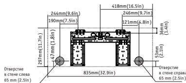
KMGA35HZRN1
