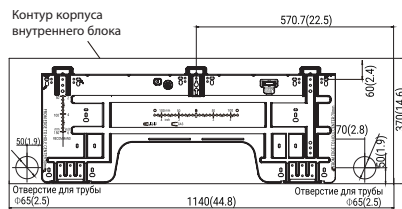
KMGP70HZRN1
