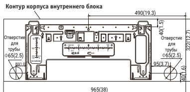
KMGP26HZRN1, KMGP35HZRN1
