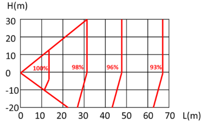
Figure 2-7.8: 180 model rate of change in heating capacity
