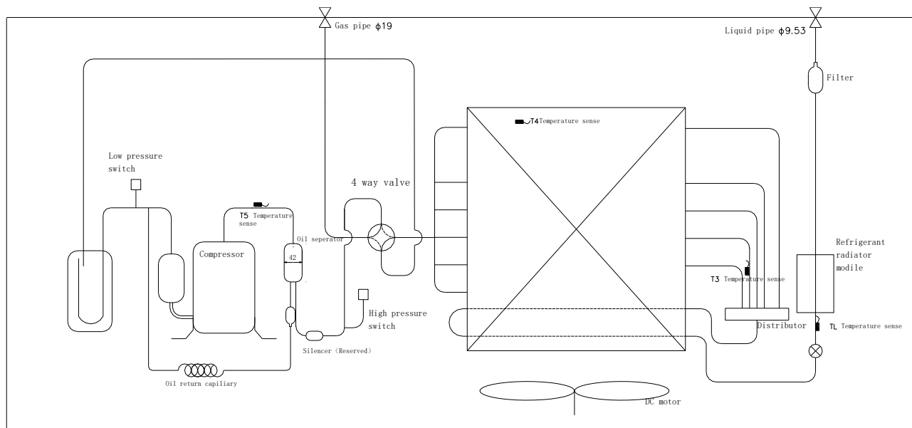
Figure 2-4.5: 18 model Piping diagram
