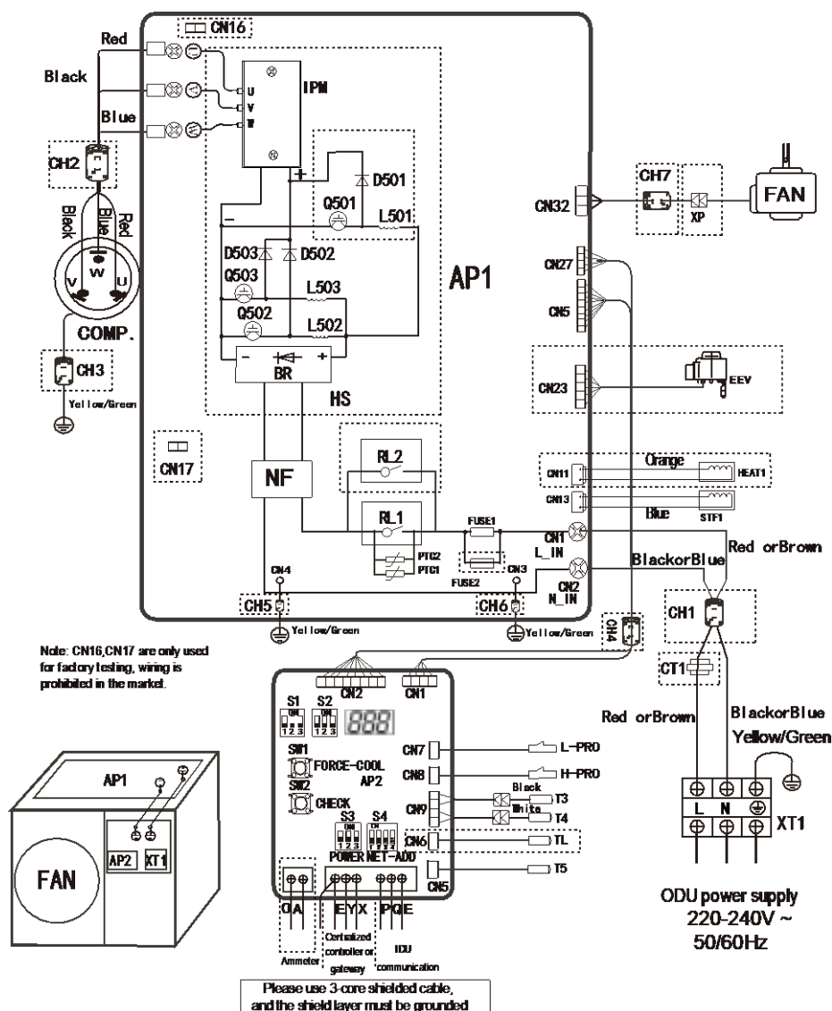
Figure 2-5.2: 100/120/140/160 model wiring diagram
