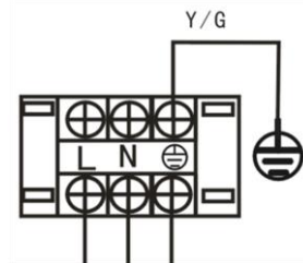
Figure 3-8.2: Outdoor unit 1-phase power supply terminals
