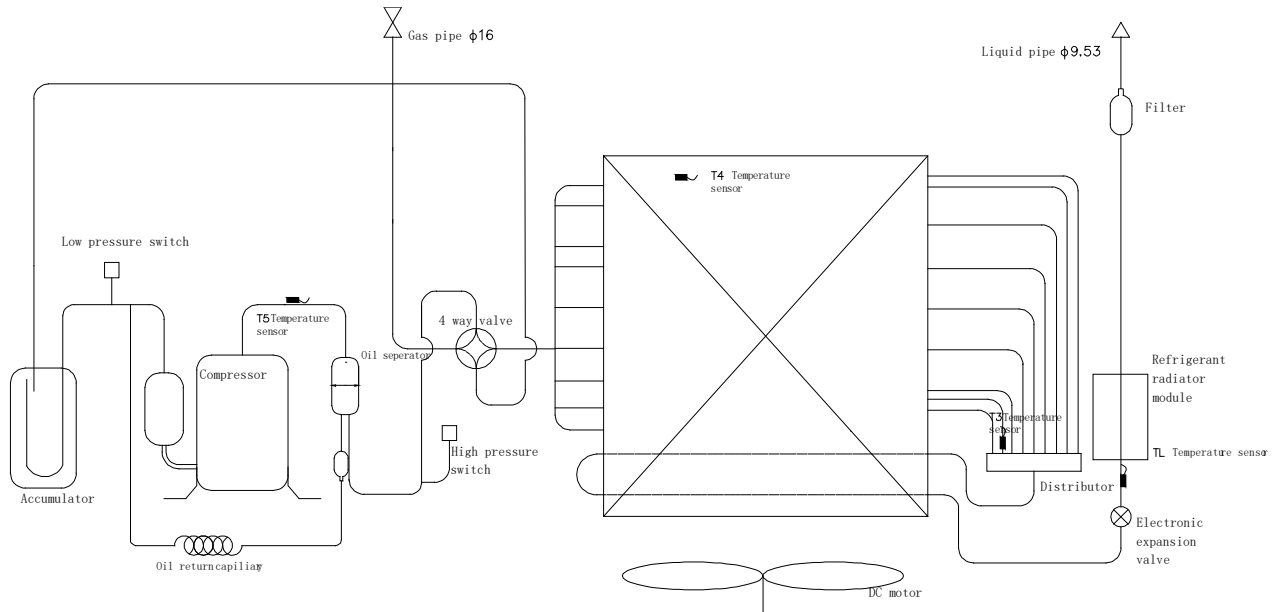
Figure 2-4.4: 140/160 model Piping diagram
