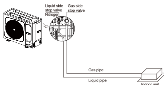
Figure 3-4.11: Gastightness test
