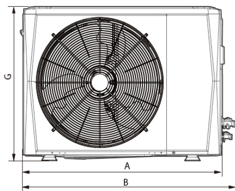
Figure 2-2.3: Model 100-160 Front view dimensions
