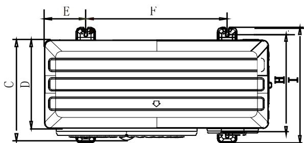
Figure 2-2.6: Model 180 Top view dimensions
