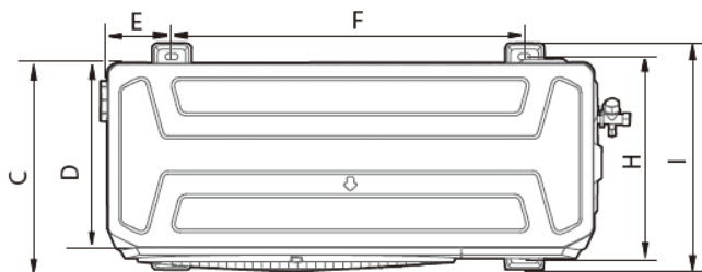
Figure 2-2.2: Model 80 Top view dimensions
