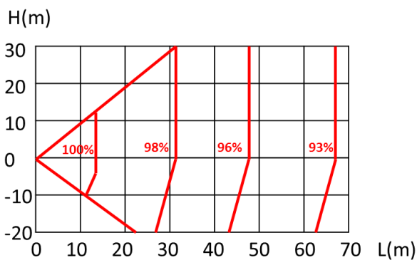
Figure 2-7.7: 180 model rate of change in cooling capacity
