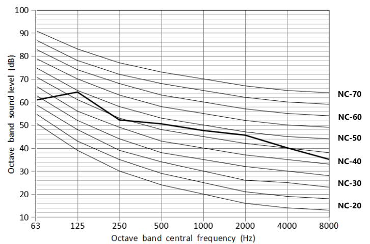
Figure 2-9.7: 180 model octave band level
