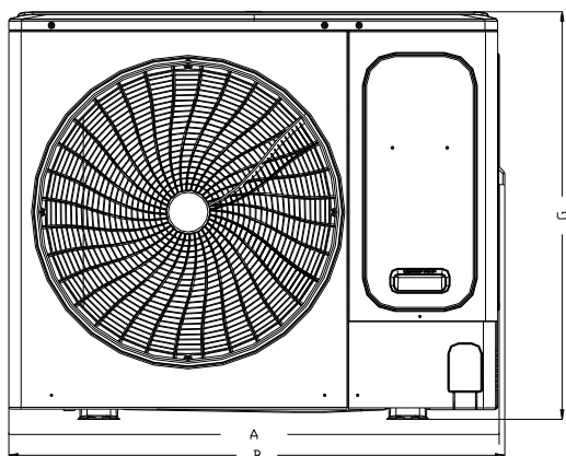
Figure 2-2.5: Model 180 Front view dimensions
