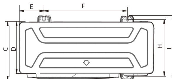
Figure 2-2.4: Model 100-160 Top view dimensions
