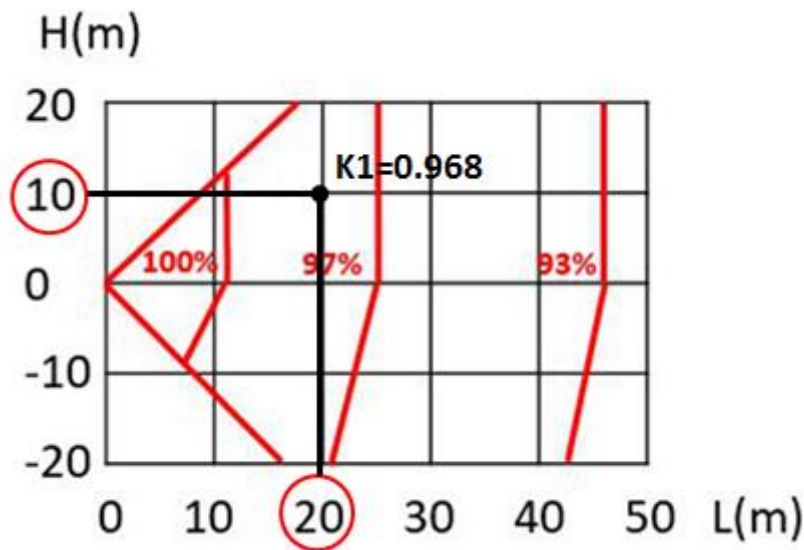
Figure 1-5.3: Outdoor unit rate of change in cooling capacity
