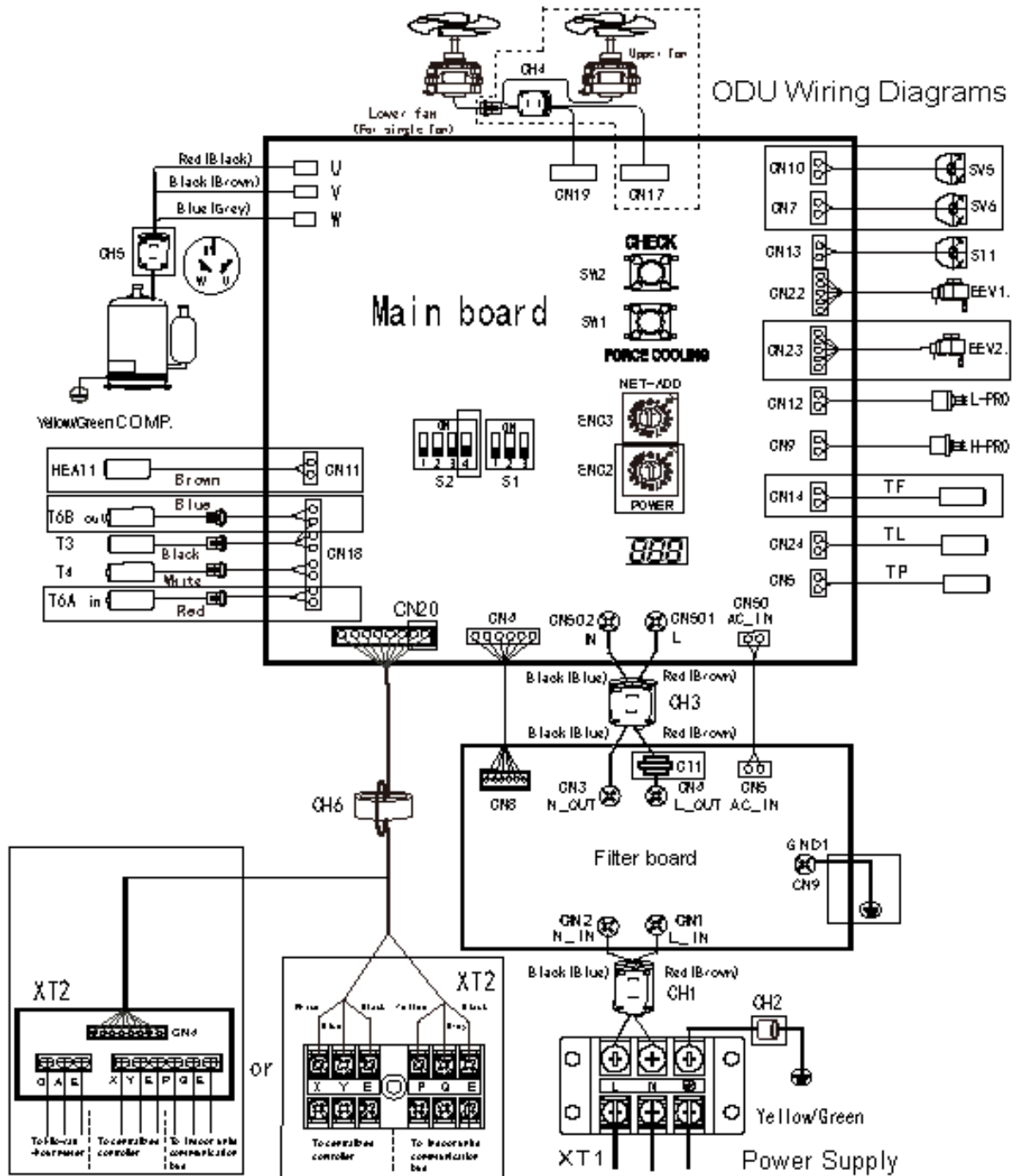
Figure 2-5.3: 180 model wiring diagram
