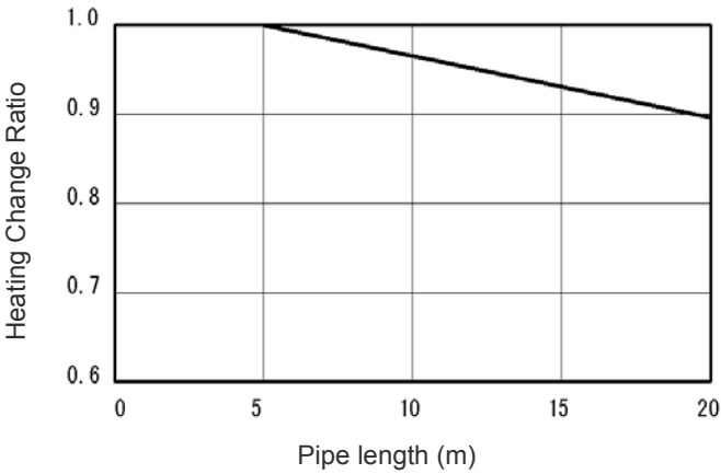
Models : RAK-DJ50PHAE/RAC-DJ50PHAE
