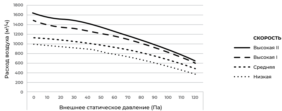
LAC-DR70HP.D01/S
