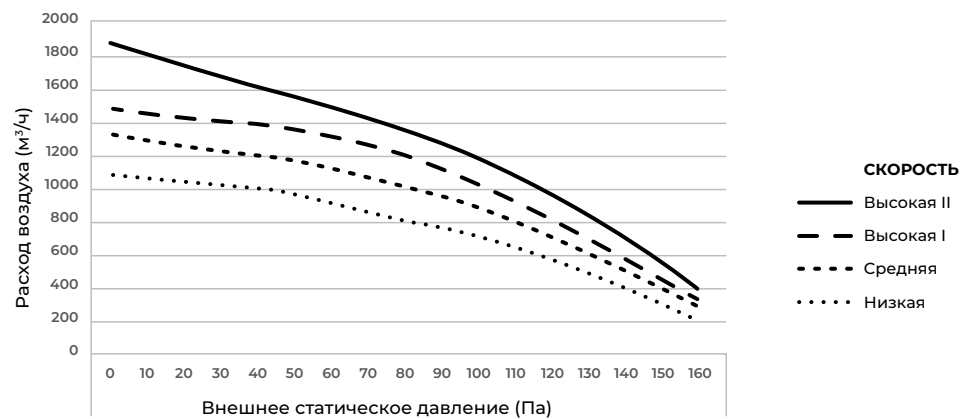
LAC-DR140HP.D01/S
