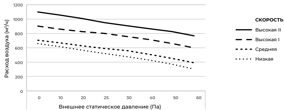
LAC-DR55HP.D01/S
