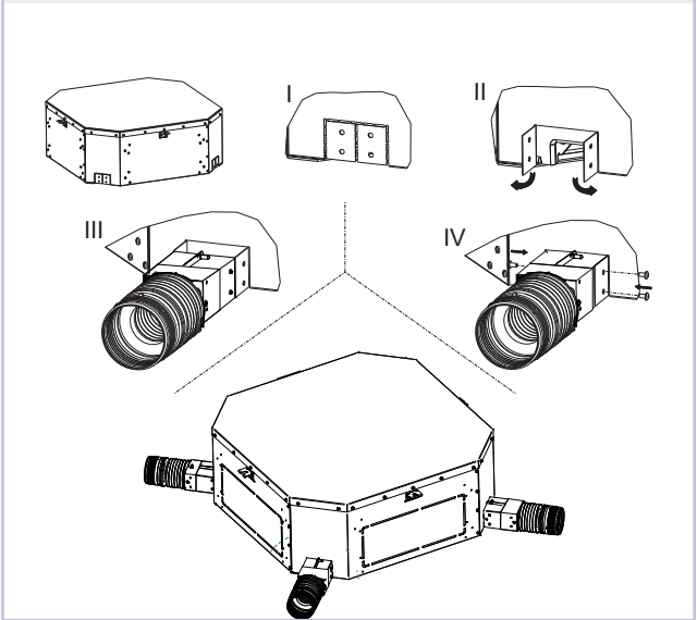
» Fig.18 FWH-A 06-07-08
