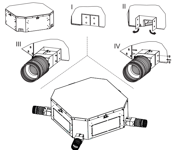
» Fig.18 FWH-A 06-07-08
