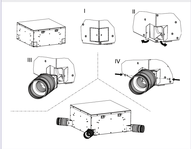
» Fig.17 FWH-A 02-03-04
