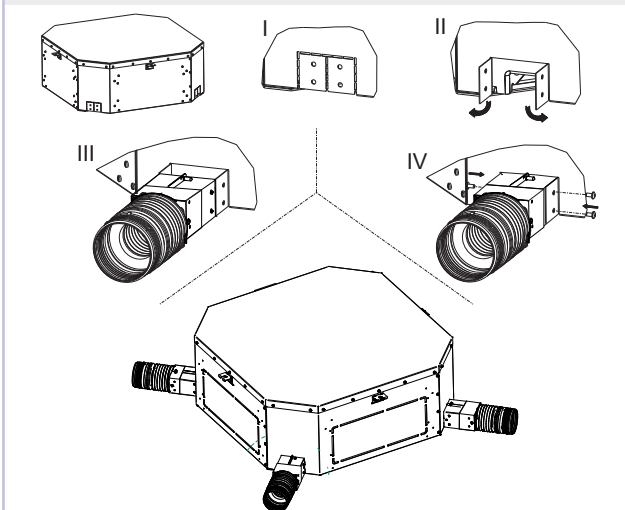
» Fig.18 FWH-A 06-07-08
