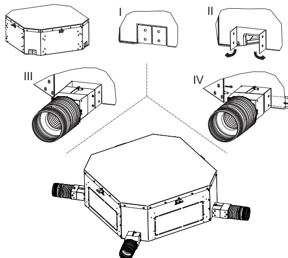
» Fig.18 FWH-A 06-07-08
