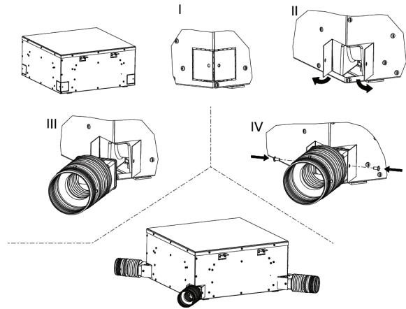
» Fig.17 FWH-A 02-03-04
