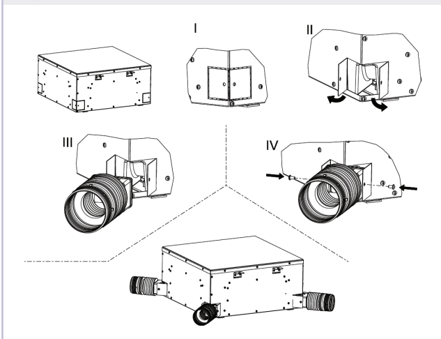
» Fig.17 FWH-A 02-03-04
