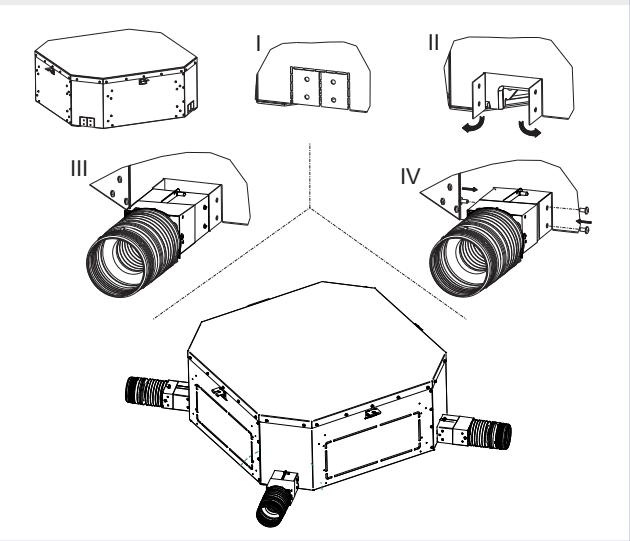
» Fig.18 FWH-A 06-07-08
