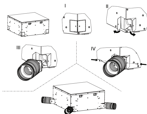
» Fig.17 FWH-A 02-03-04
