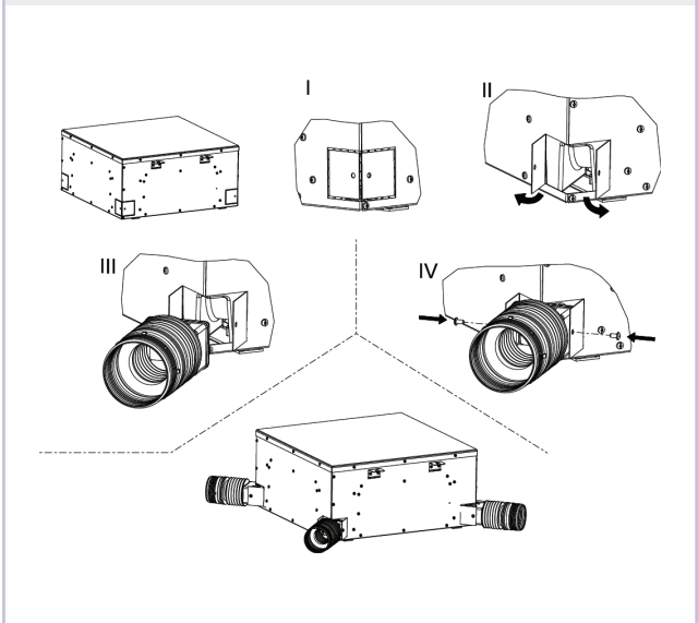
» Fig.17 FWH-A 02-03-04
