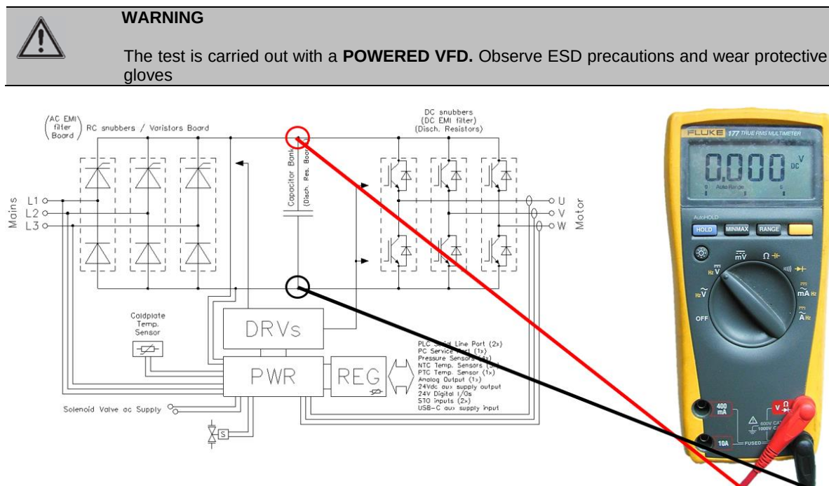
Figure 43 DC-BUS Voltage measurement
