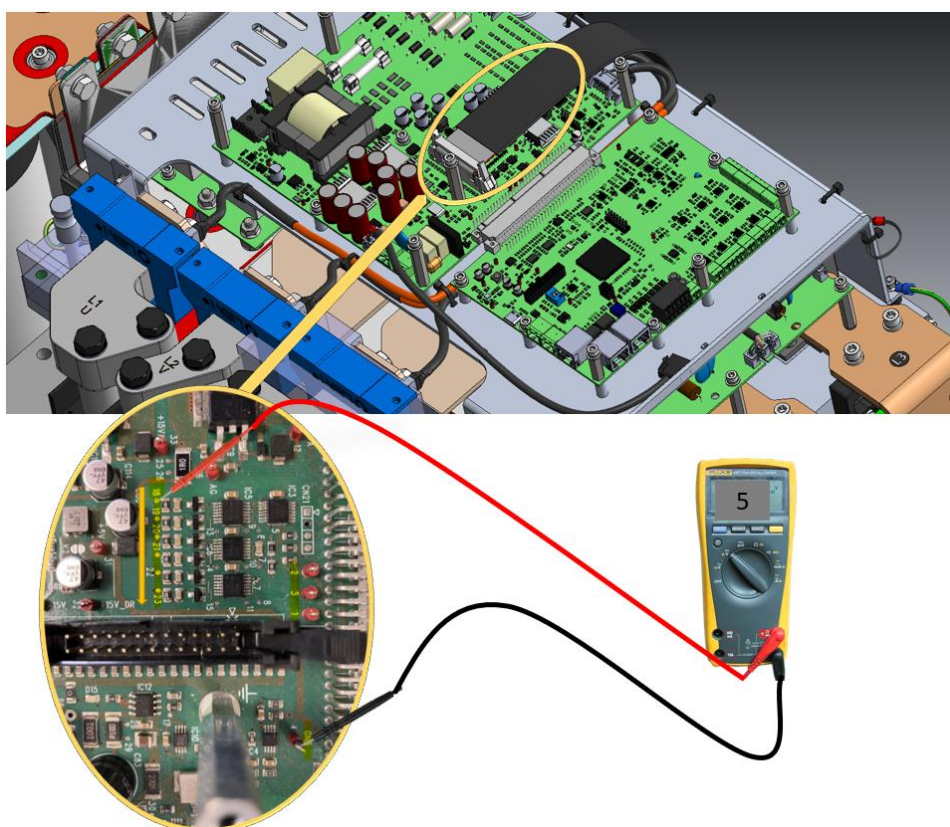
Figure 35 POWER CARD Check: 5V DC on 18 – 23 spots
