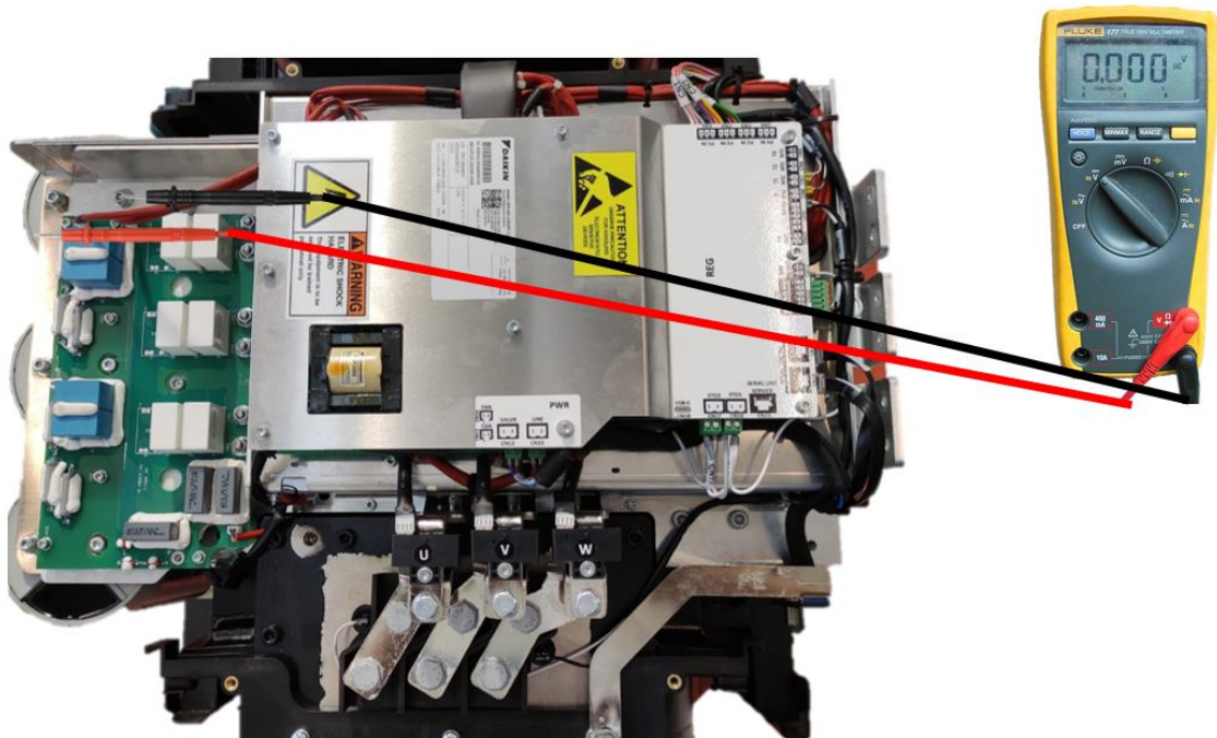
Figure 77 200 kW DAE VFD - DC-BUS Check
