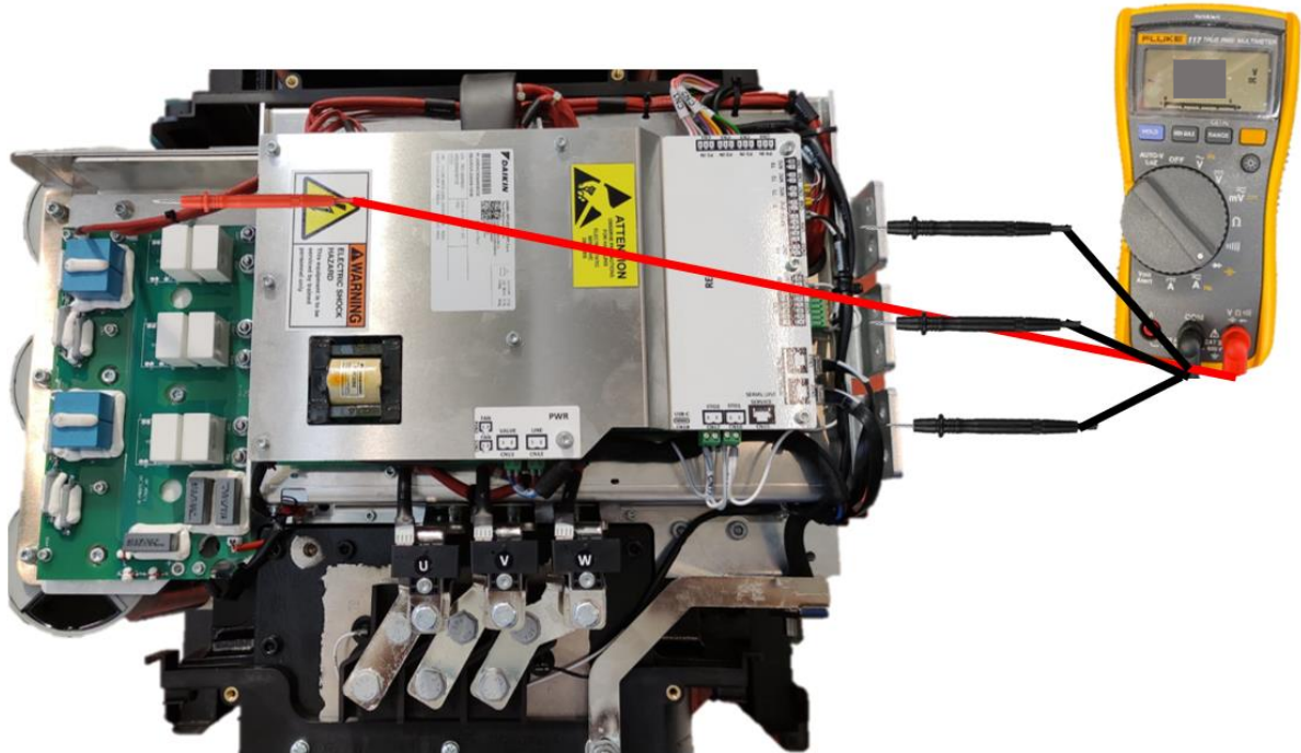
Figure 78 200 kW DAE VFD – Bottom SCR Direct polarization
