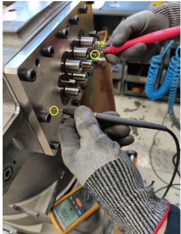
Figure 39 Electrical insulation terminal thermistor - earth
