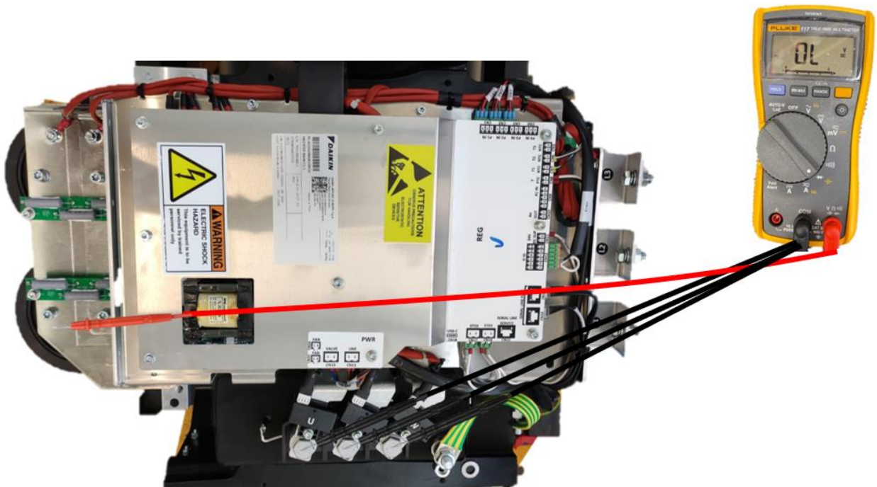
Figure 76 90 kW -120 kW DAE VFD - TOP IGBT Indirect polarization
