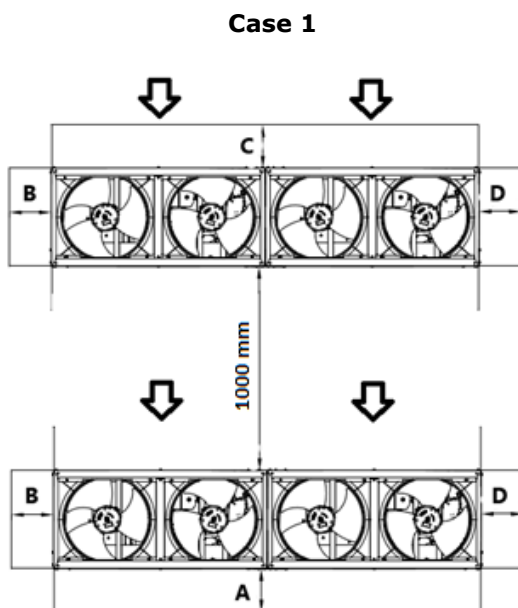
Units installed side by side along their longer sides (Case 1 and Case 2)
