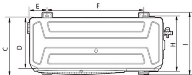
Figure 2-2.2: Model 80 - 100 Top view dimensions
