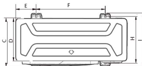
Figure 2-2.4: Model 120-160 Top view dimensions
