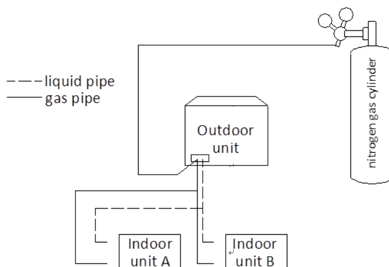
Figure 3-4.9: Pipe flushing using nitrogen
