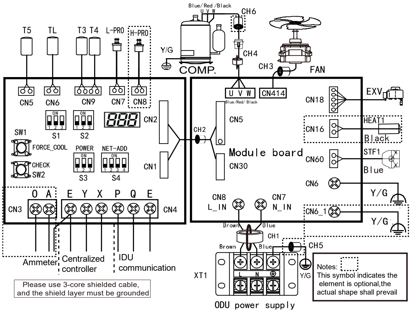
Figure 2-5.1: 80 model wiring diagram
