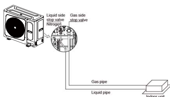
Figure 3-4.11: Gastightness test
