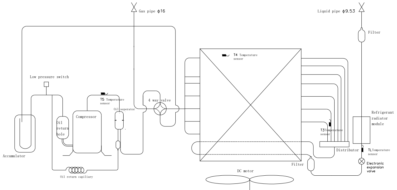
Figure 2-4.1: 80 model Piping diagram
