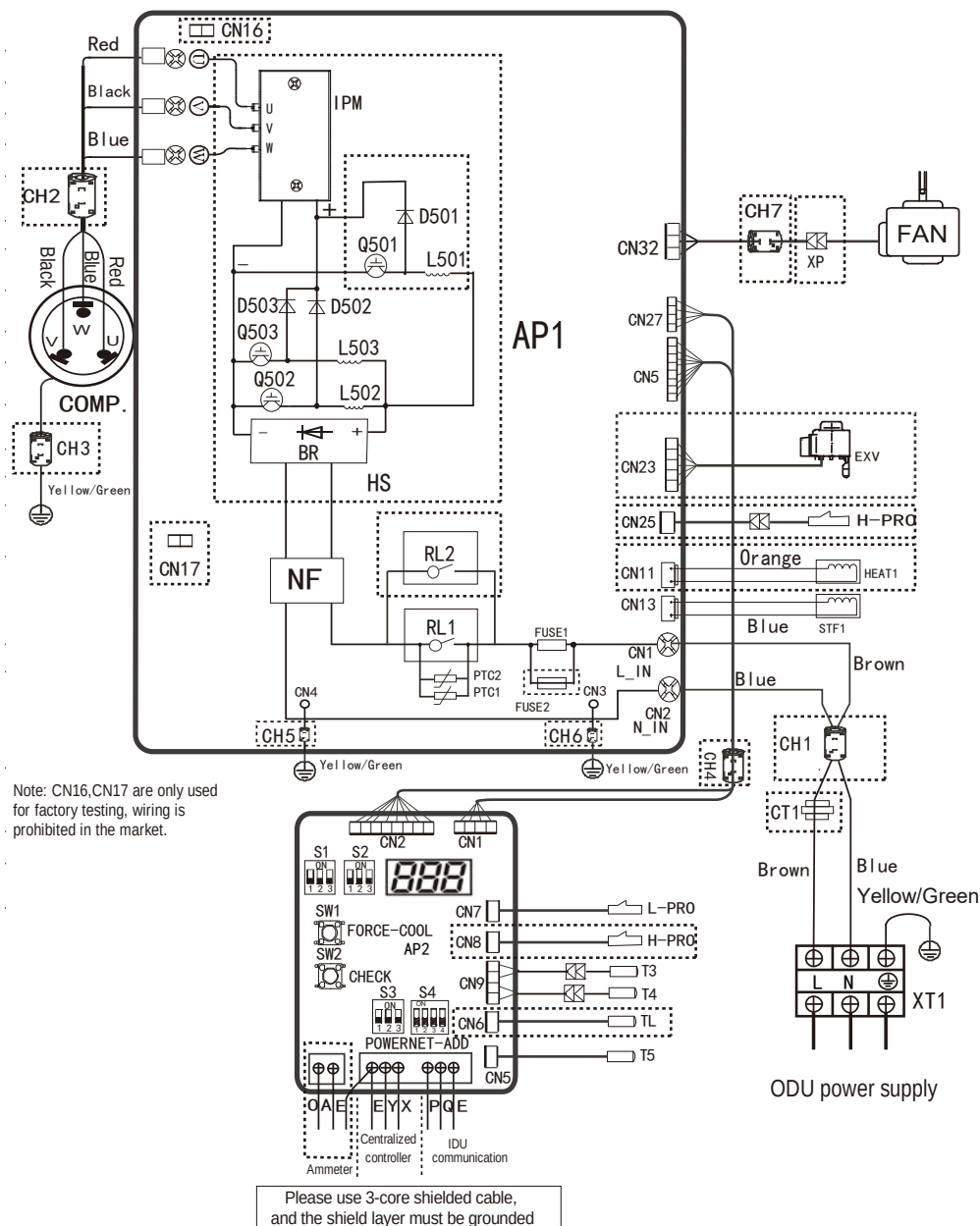
Figure 2-5.2: 100 / 120 / 140 / 160 model wiring diagram
