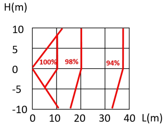
Figure 2-7.3: 100 model rate of change in cooling capacity
