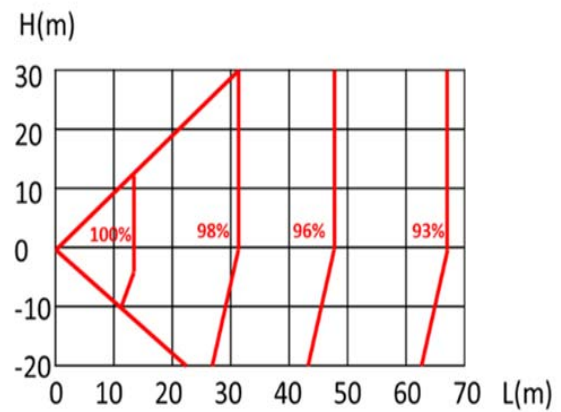
Figure 2-7.7: 140 / 160 model rate of change in cooling capacity
