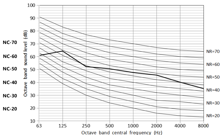
Figure 2-9.5: 140 model octave band level
