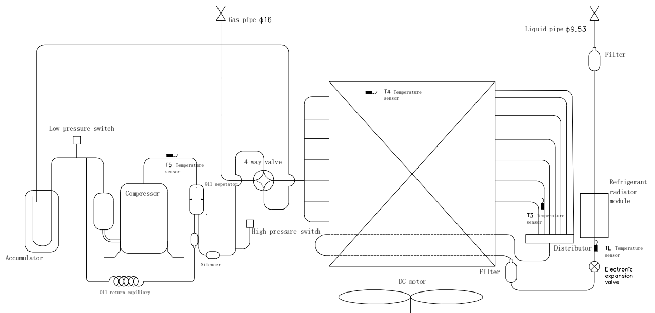
Figure 2-4.2: 100 model Piping diagram
