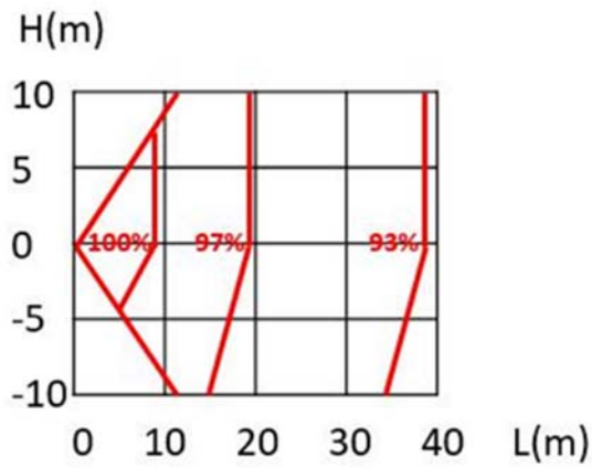
Figure 2-7.1: 80 model rate of change in cooling capacity
