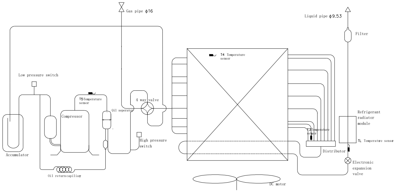
Figure 2-4.3: 120 model Piping diagram
