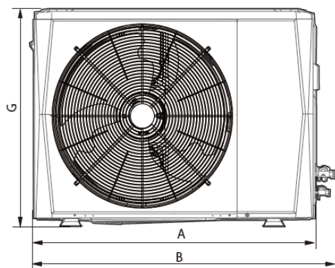
Figure 2-2.1: Model 80 - 100 Front view dimensions
