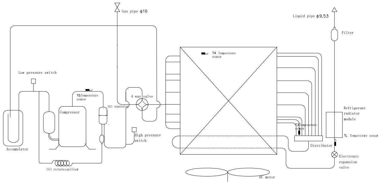
Figure 2-4.4: 140 - 160 model Piping diagram
