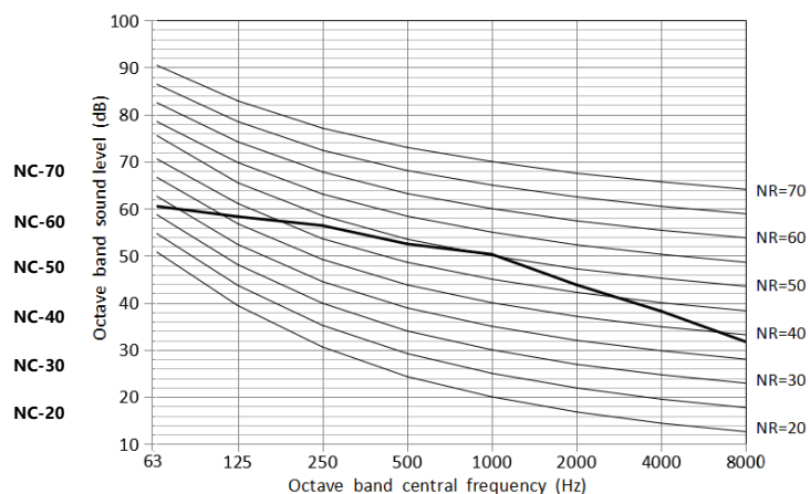
Figure 2-9.1: 80 model octave band level
