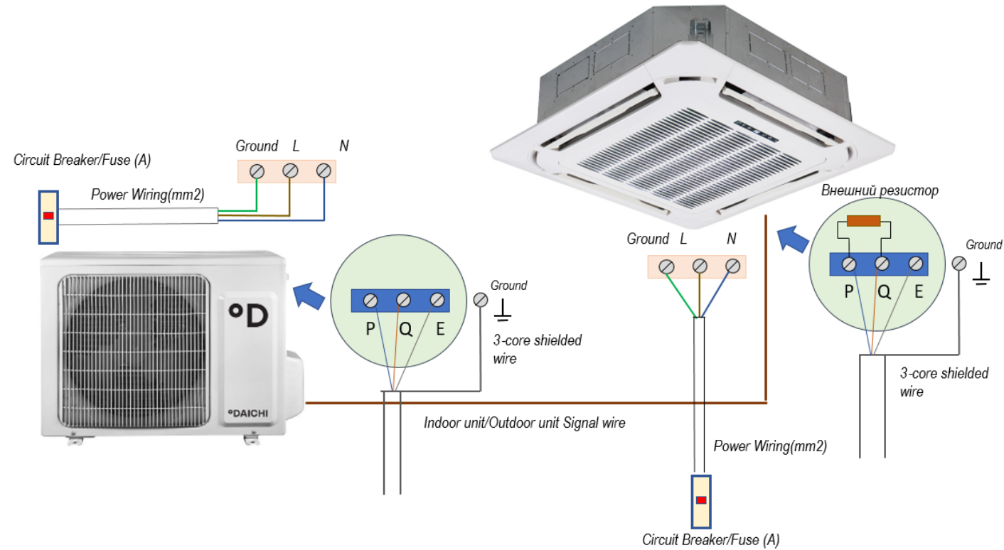
Figure 3-8.4: System power wiring example
