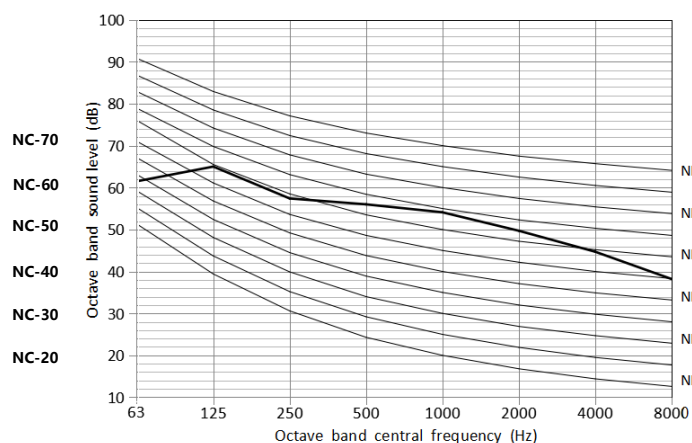
Figure 2-9.3: 120 model octave band level
