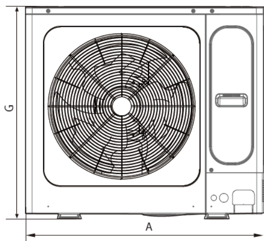
Figure 2-2.3: Model 120-160 Front view dimensions
