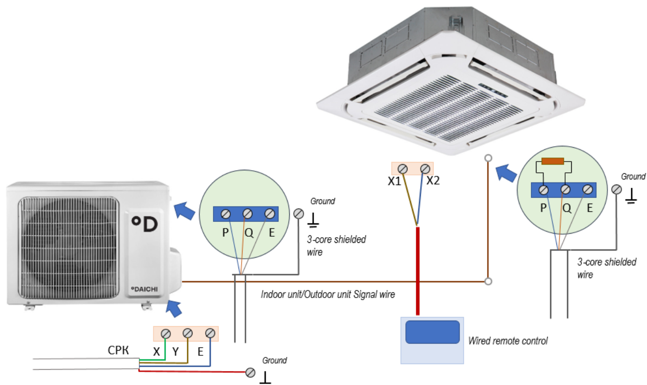
Figure 3-8.4: System communication wiring example
