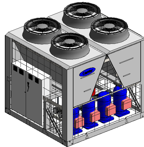
30RB-RBP Revit Family in Project Environment
