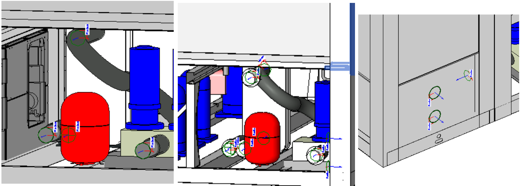
Connectors at Inlet and Outlet Connections of the unit ( Hydronic Kit, BPHE piping and Buffer Tank)
