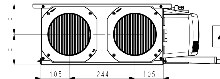
42NX T2/T3/T4 MANCHETTE / RECTANGULAR FLANGE
