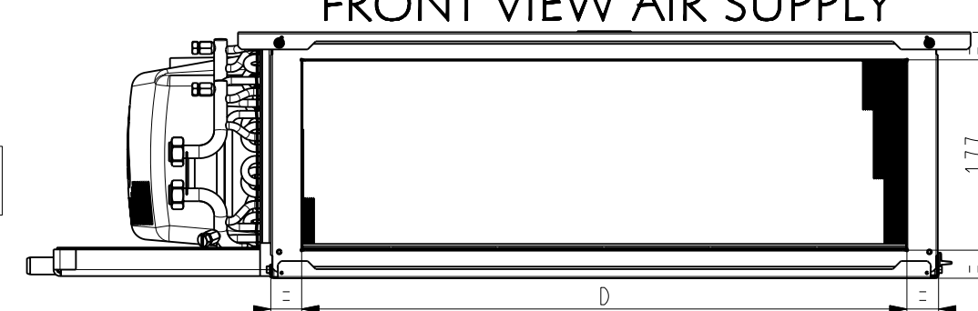
42NX T2/T3/T4 MANCHETTE / RECTANGULAR FLANGE
