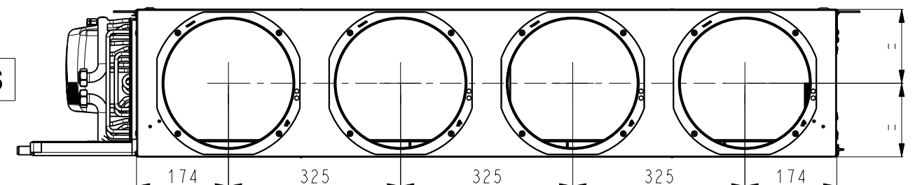
VIROLES / SPIGOTS Ø250
