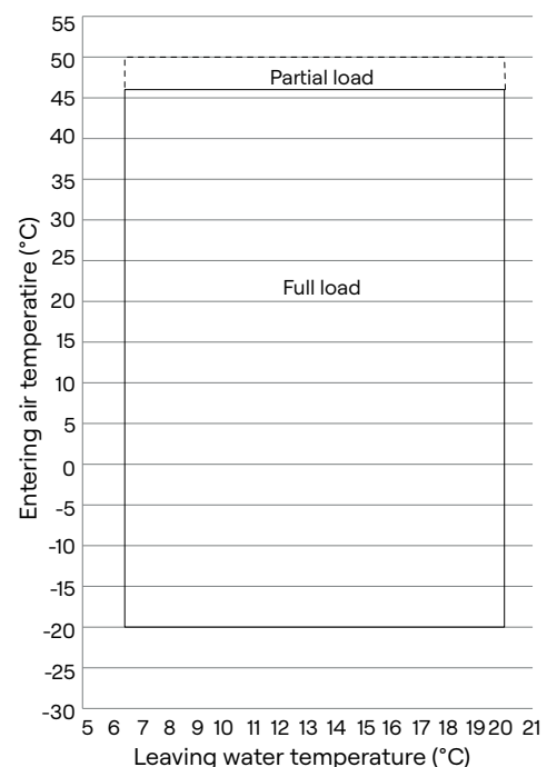
Operating map - cooling mode Standard unit 61AQ
