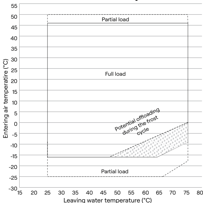
Operating map - heating mode Standard unit 61AQ
