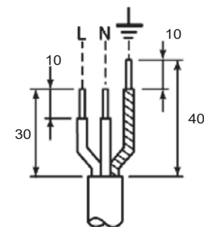
Power supply connection diagram
