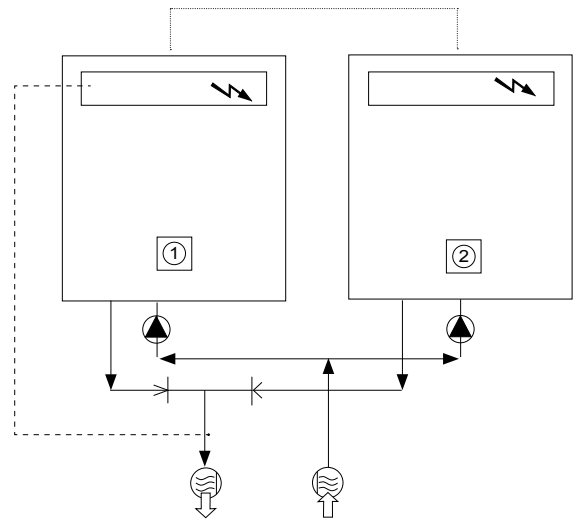
30XW with configuration: leaving water control
