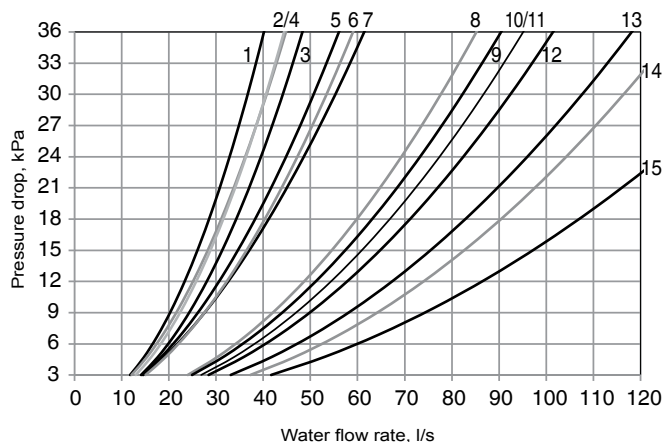
Units with one evaporator pass (option 100C): 30XW--/30XWH-/30XW-P/30XWHP
