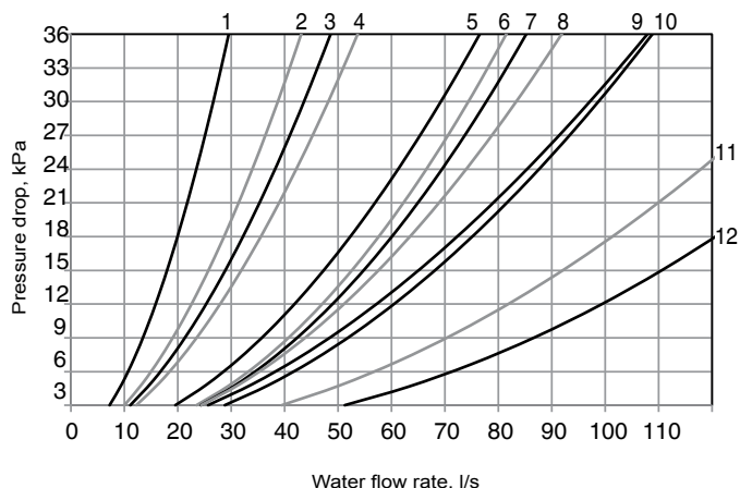
Units with one condenser pass (option 102C): 30XW--/30XWH-/30XW-P/30XWHP
