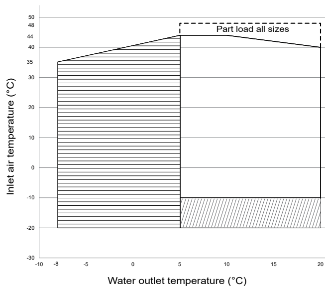
Operating map - unit 30RB option 16 30RB 040R-160R
