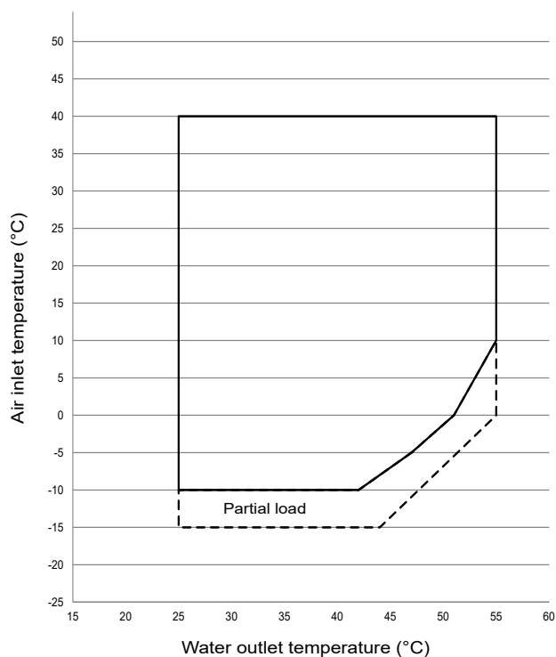
Operating map - heating mode - Standard unit 30RQ
