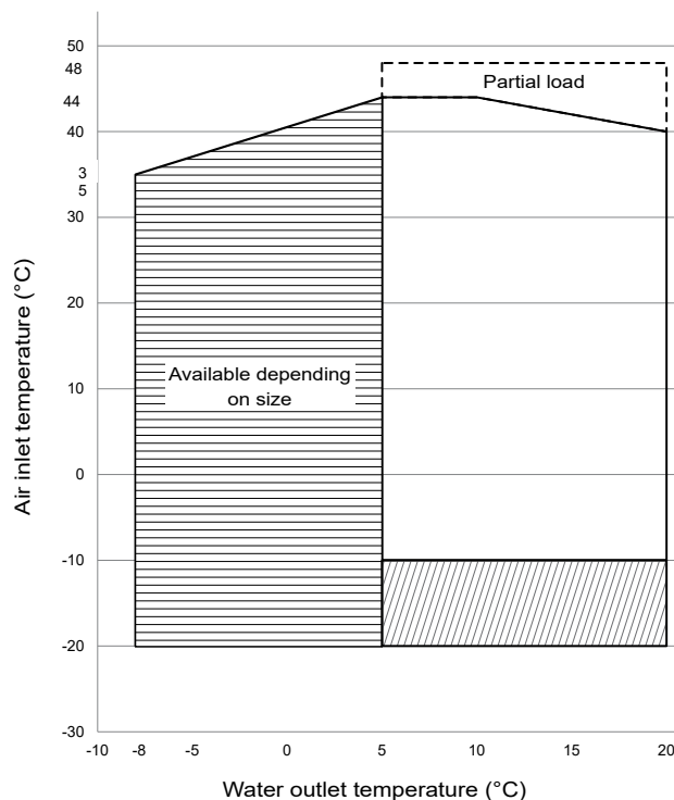
Operating map - cooling mode - 30RQ unit option 16
