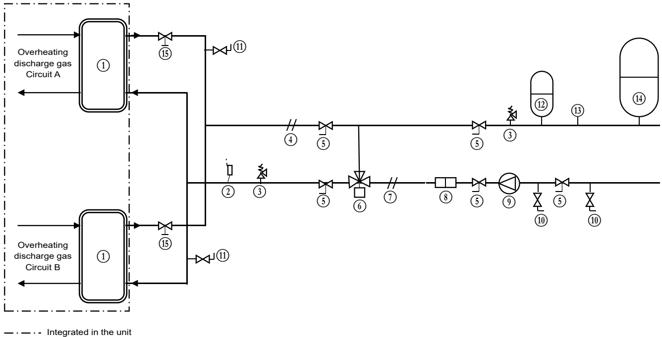
Typical installation diagram of units with the desuperheater option
