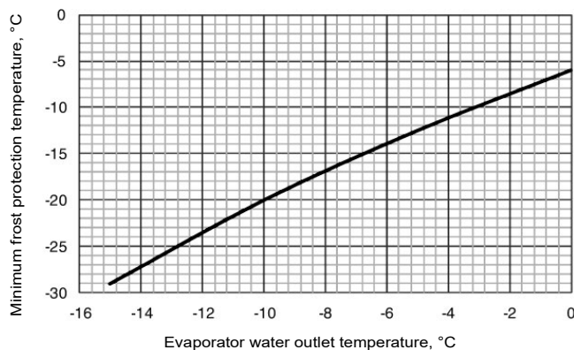
Minimum frost protection activation temperature
