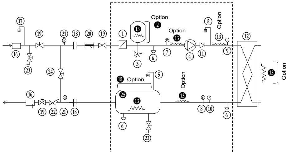
Schematic diagram of the hydraulic circuit with the hydraulic module
