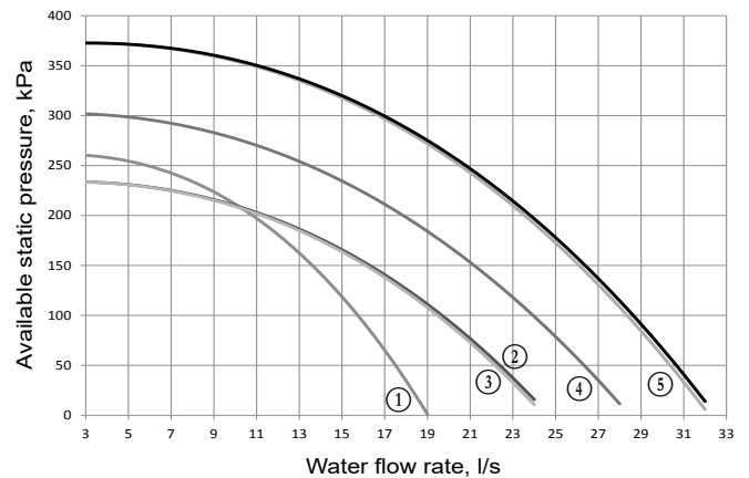
Dual pump high pressure
