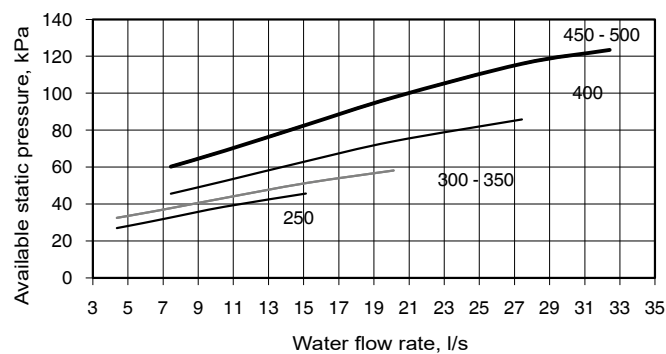
High-pressure pumps (options 116R/116S)
