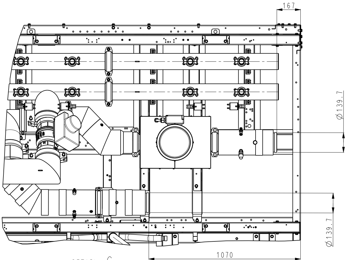
DETAIL C ECHELLE 21:320
