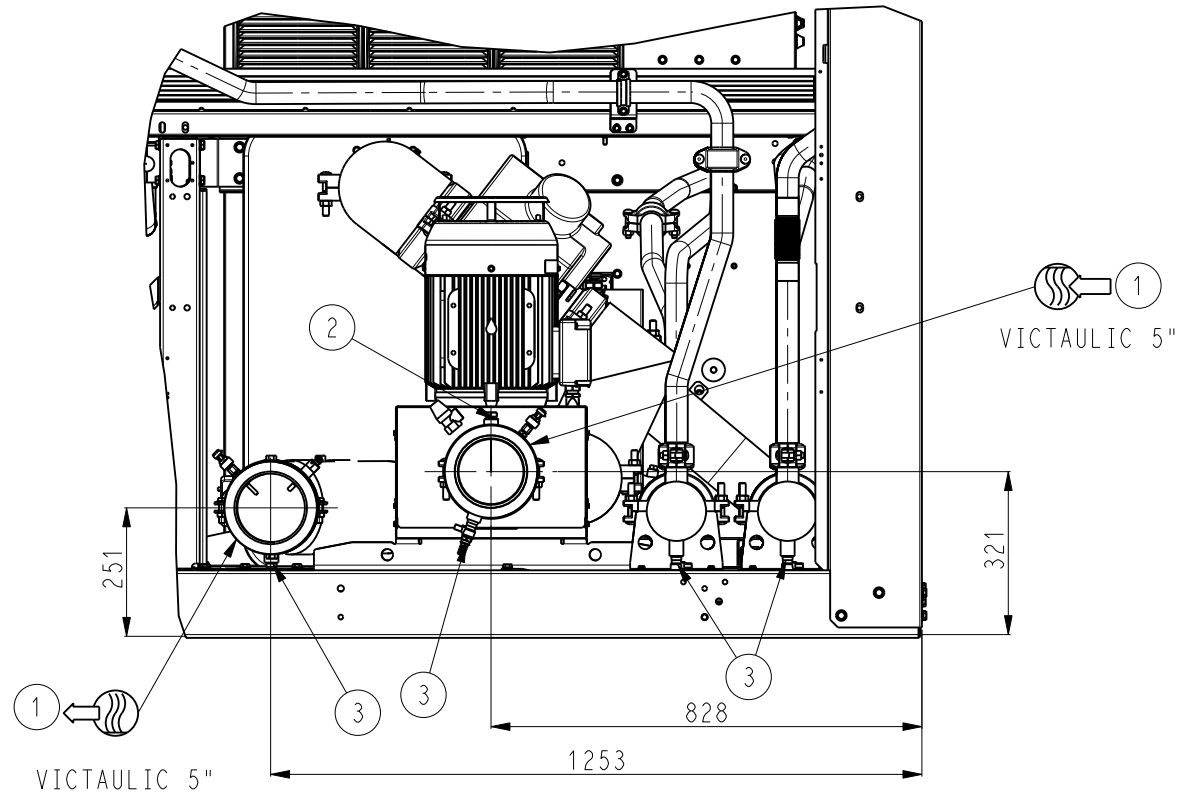
VCE G VIEW ECHELLE 11:160
