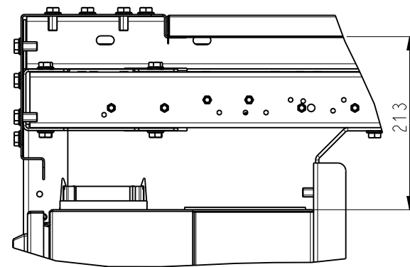
DETAIL H ECHELLE 3:20
