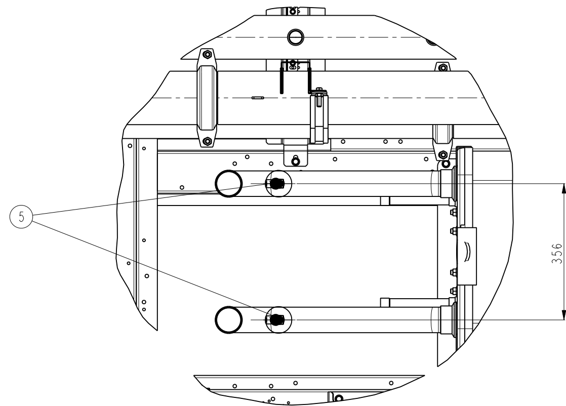
DETAIL B ECHELLE 1:10
