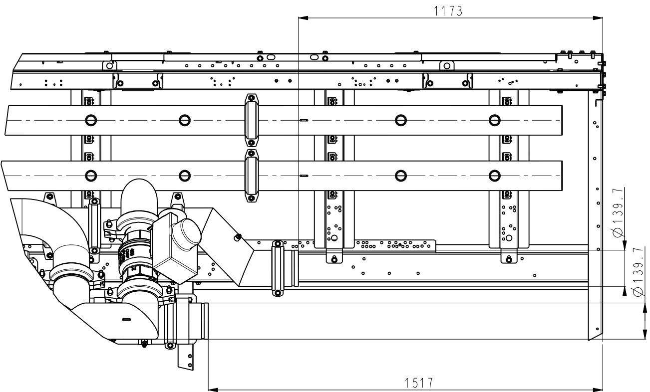
DETAIL C ECHELLE 11:160
