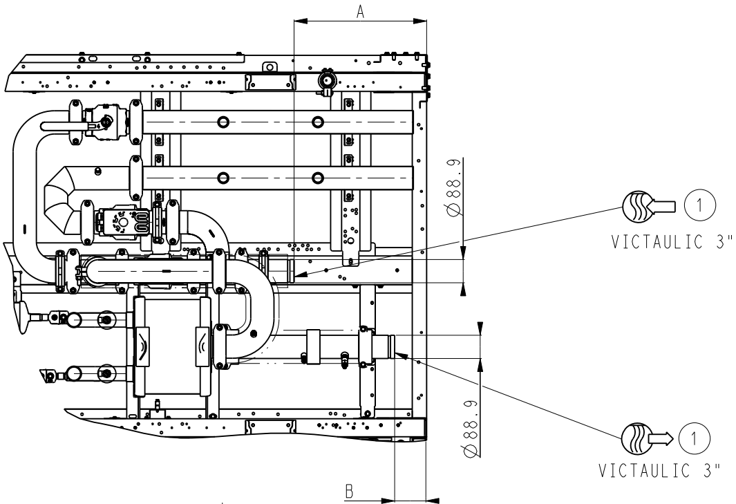
DETAIL J ECHELLE 1:20
