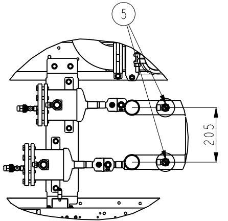
DETAIL C ECHELLE 11:160
