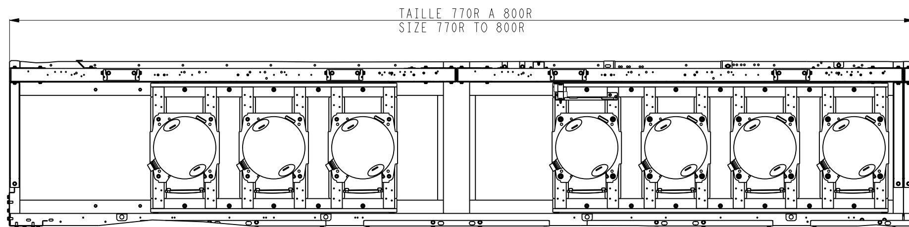
DETAIL C ECHELLE 11:160
