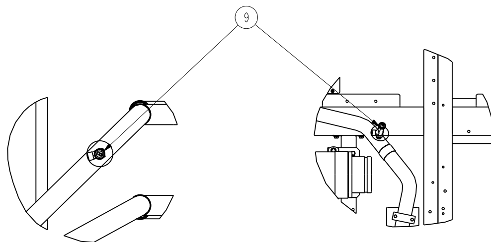
DETAIL D ECHELLE 1:10
