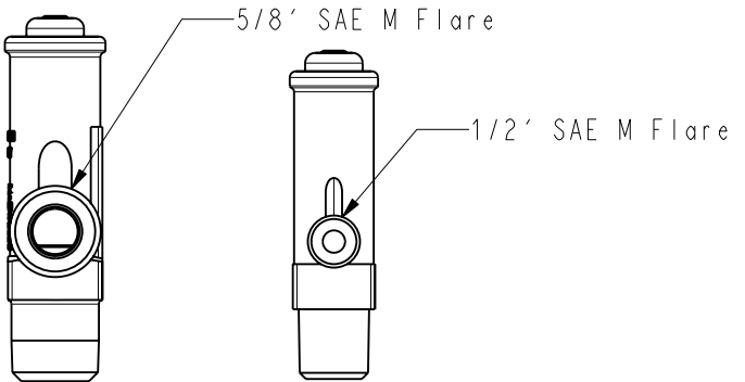
DETAIL SOUPAPE 5 DETAIL SOUPAPE 9
