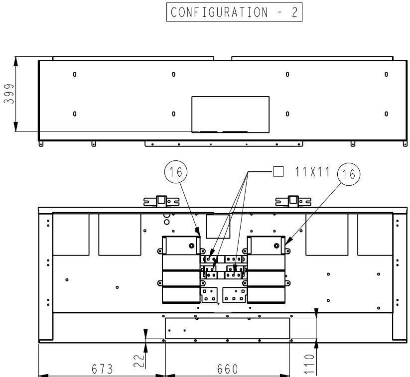
ELECTRICAL BOX: POWER CONNECTION
