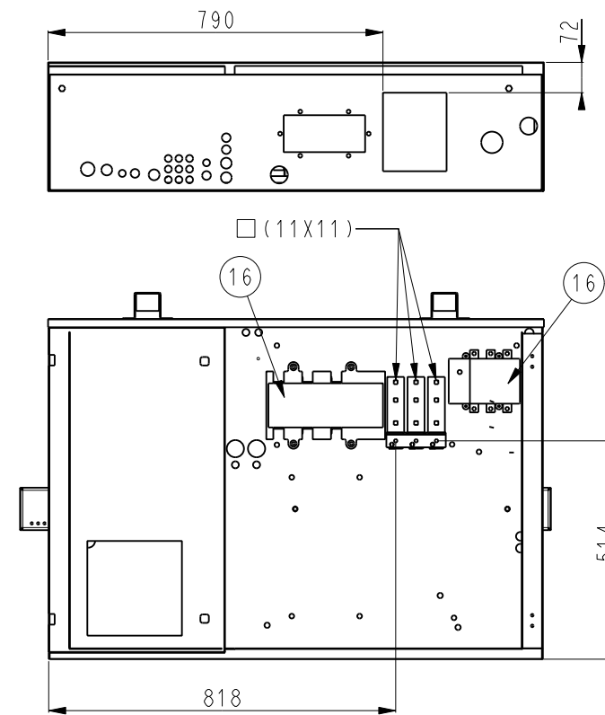
A100 ELECTRICAL BOX: POWER CONNECTION
