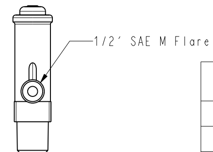
DETAIL SOUPAPE 9
