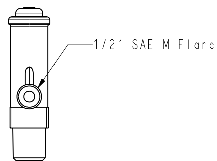
DETAIL SOUPAPE 9
