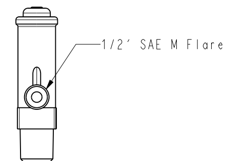
DETAIL SOUPAPE 9
